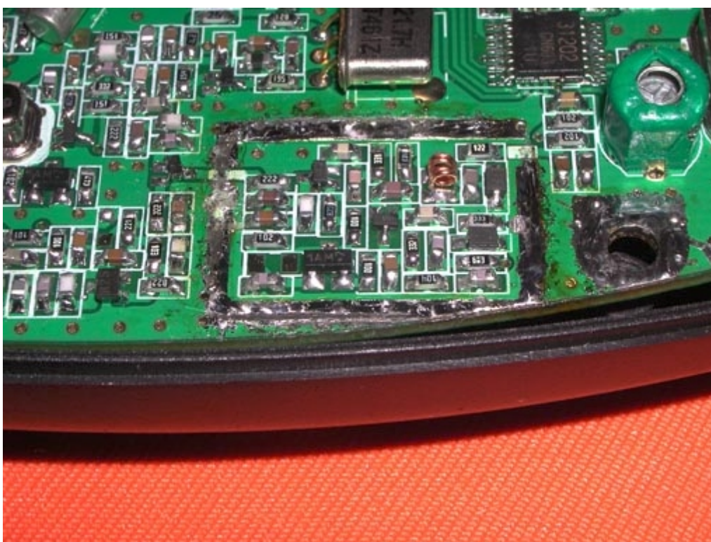
Internal Photo - 2
