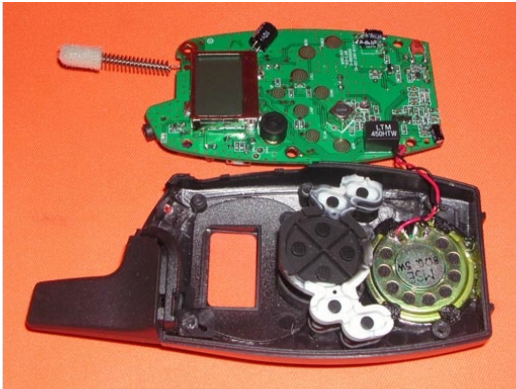
Internal Photo - 4
