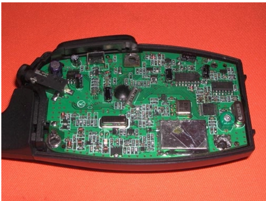
Internal Photo - 2
