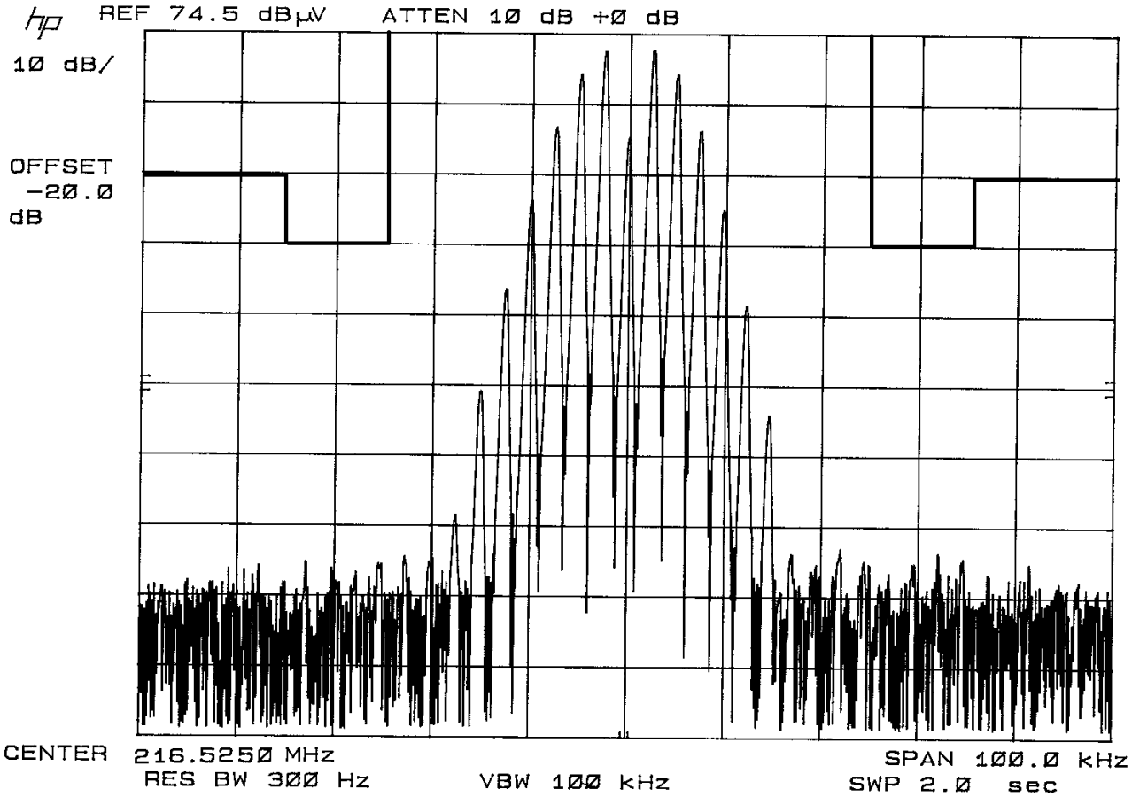
Occupied Bandwidth Plot 50 kHz channel
