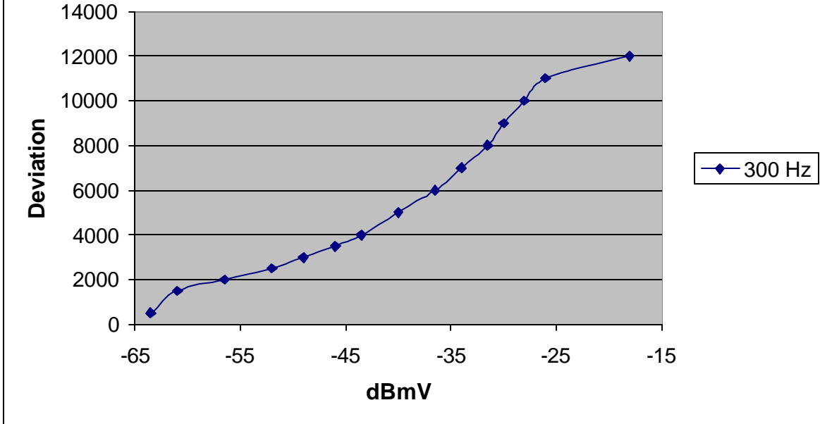
Modulation limiting 300 Hz
