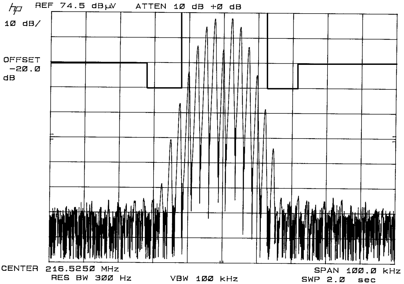
Occupied Bandwidth Plot 25 kHz channel
