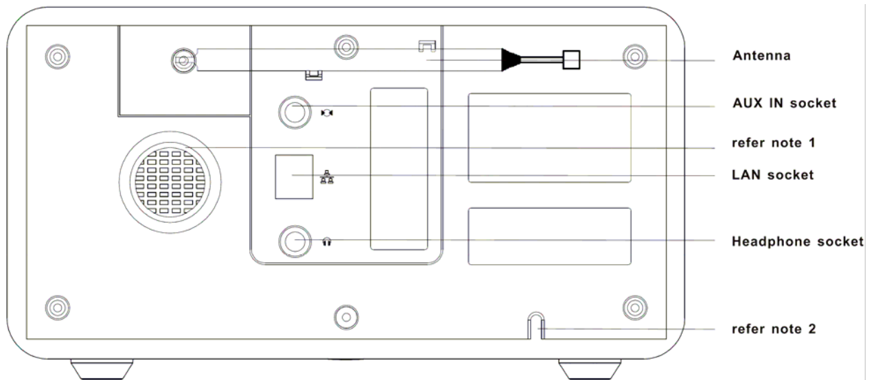
Digital Radio Back View
