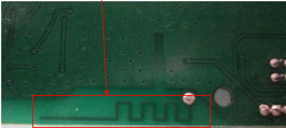
Bluetooth Antenna
