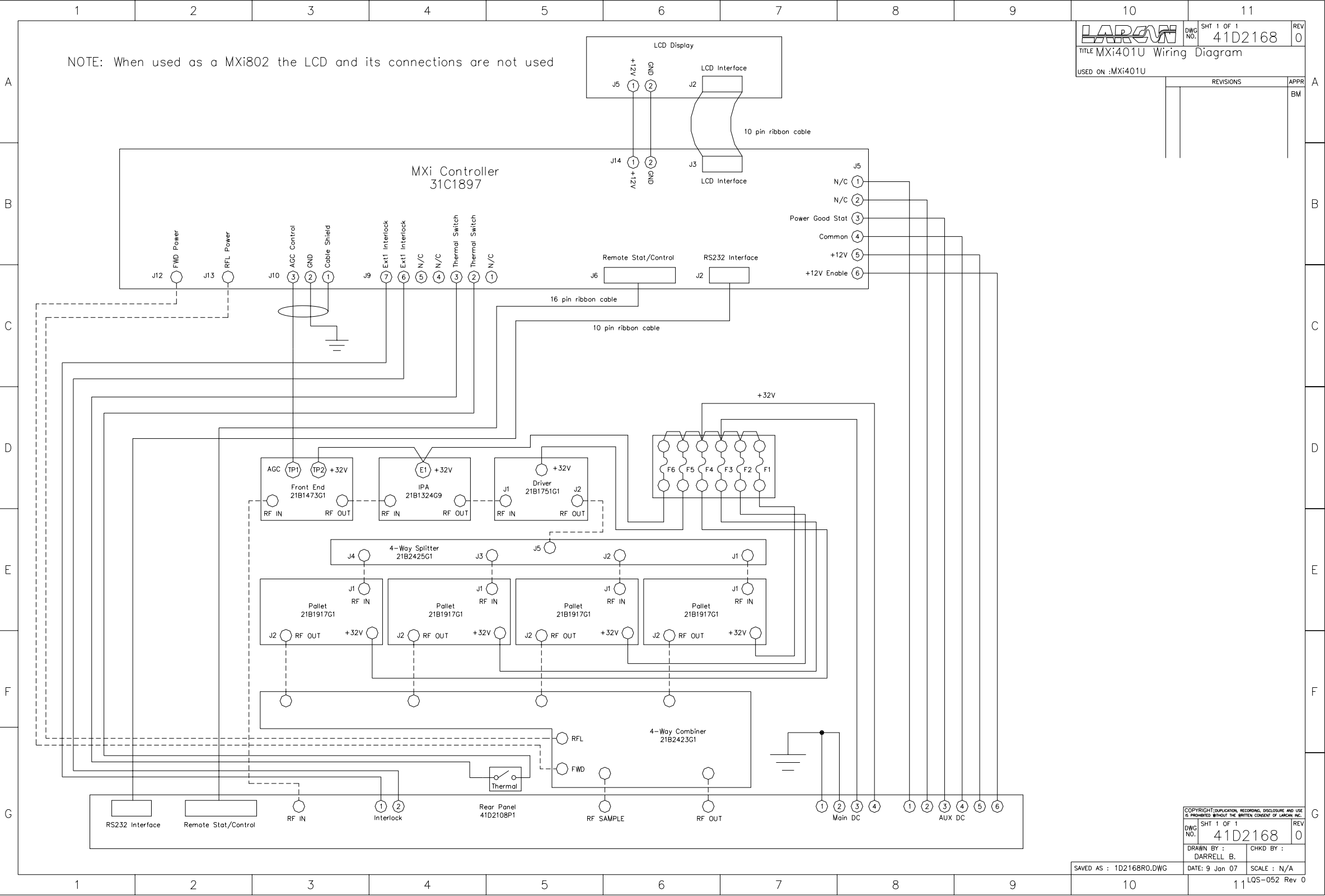
Figure 5 41D2168 MXi401/802 Amplifier Wiring Schematic sht1 Rev 0
