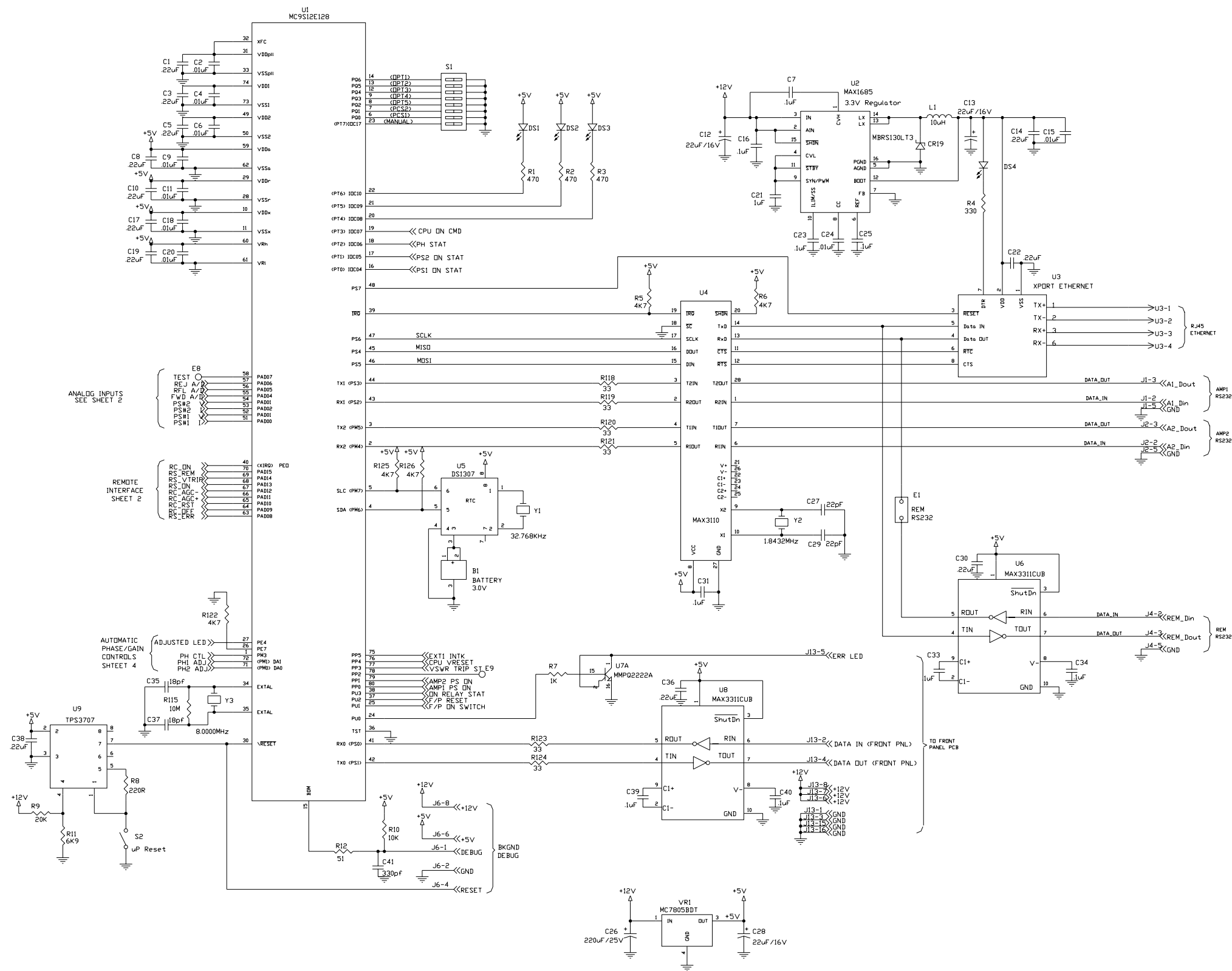
Figure 30 MXi Controller Board Schematic 31C1936 sht1 Rev 1.0
