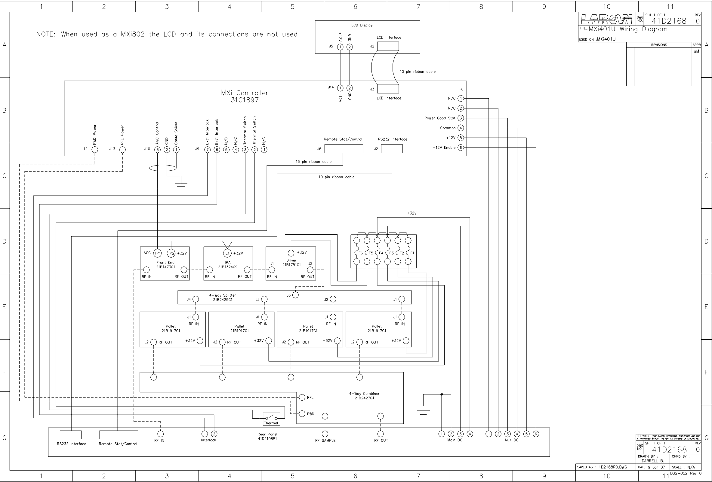
Figure 5 41D2168 MXi401U/802U Amplifier Wiring Schematic sht1 Rev 0
