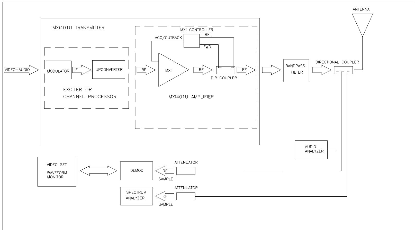
Figure 15 Test Equipment Setup
