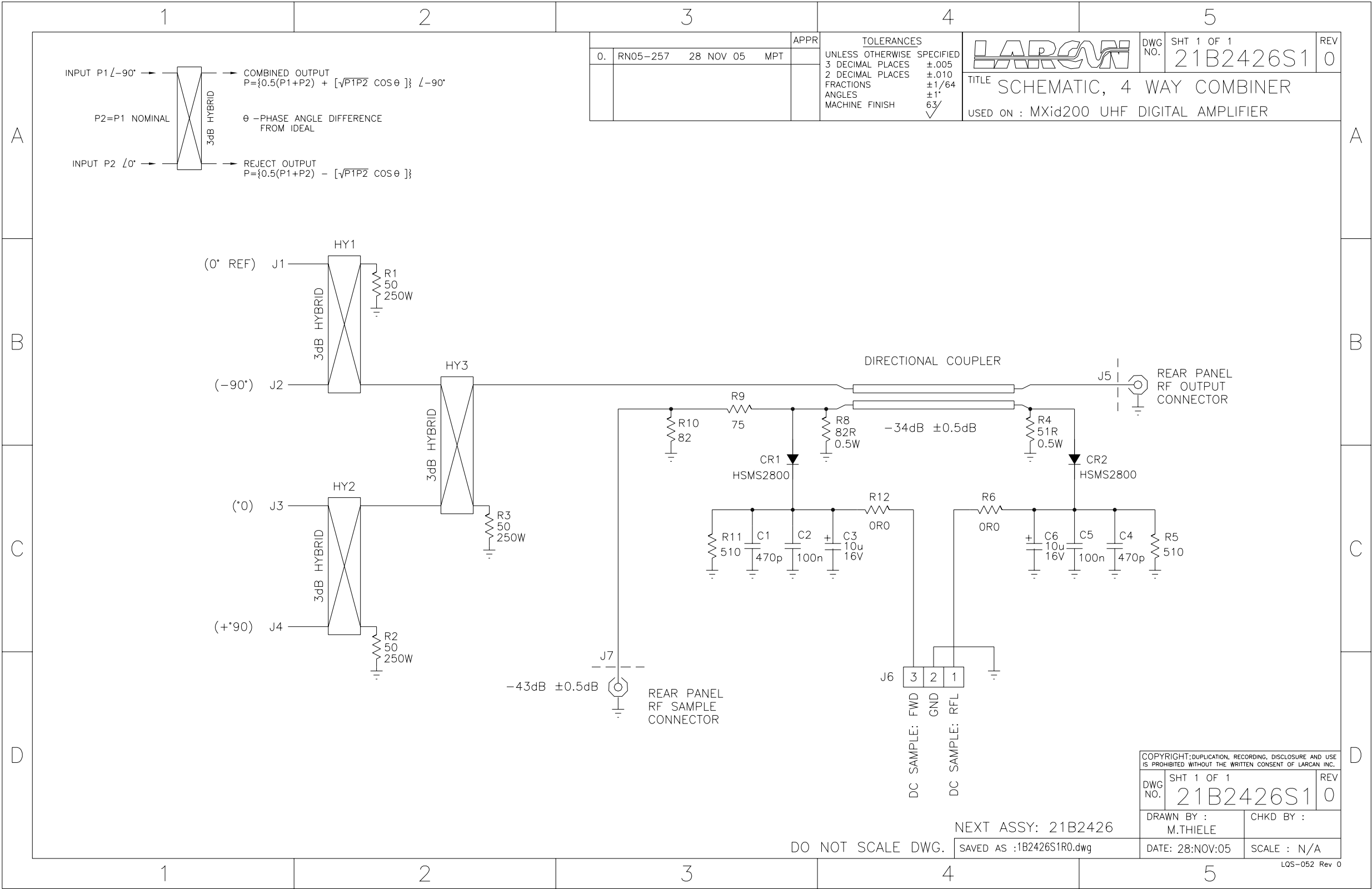
Figure 18 21B2425S1 4 Way Combiner Schematic sht1 Rev 0
