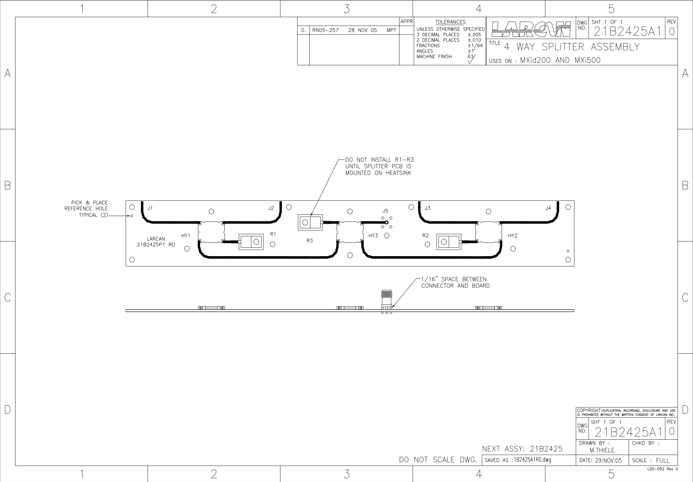
Figure 15 21B2425A1 4 Way Splitter Assembly sht1 Rev 0
