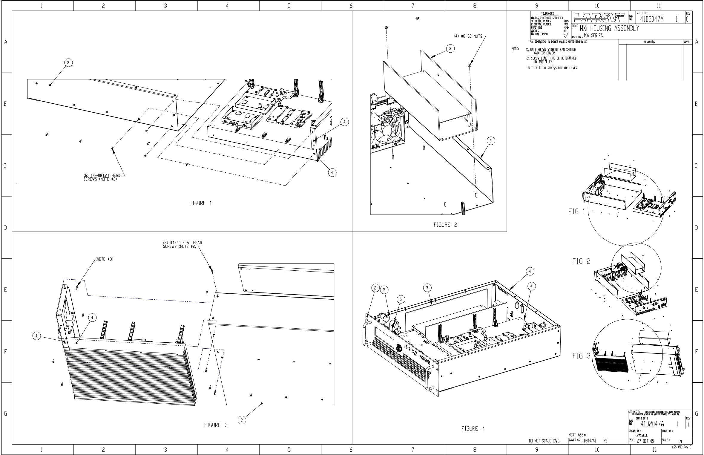
Figure 5 41D2047A1 MXi Assembly Diagram sht1 Rev 0
