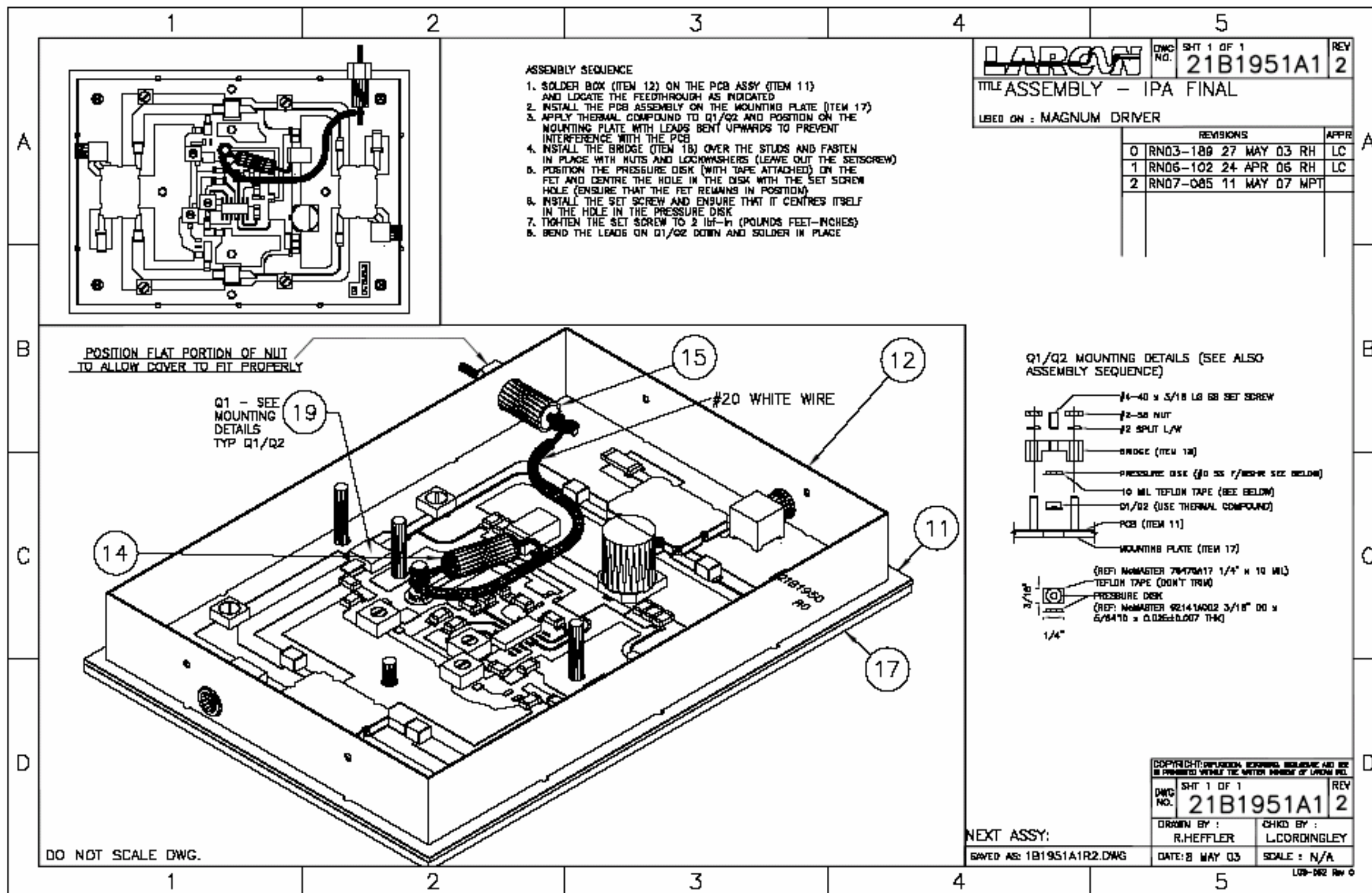
Figure 10 21B1951 IPA Final Assembly sht1 Rev 2
