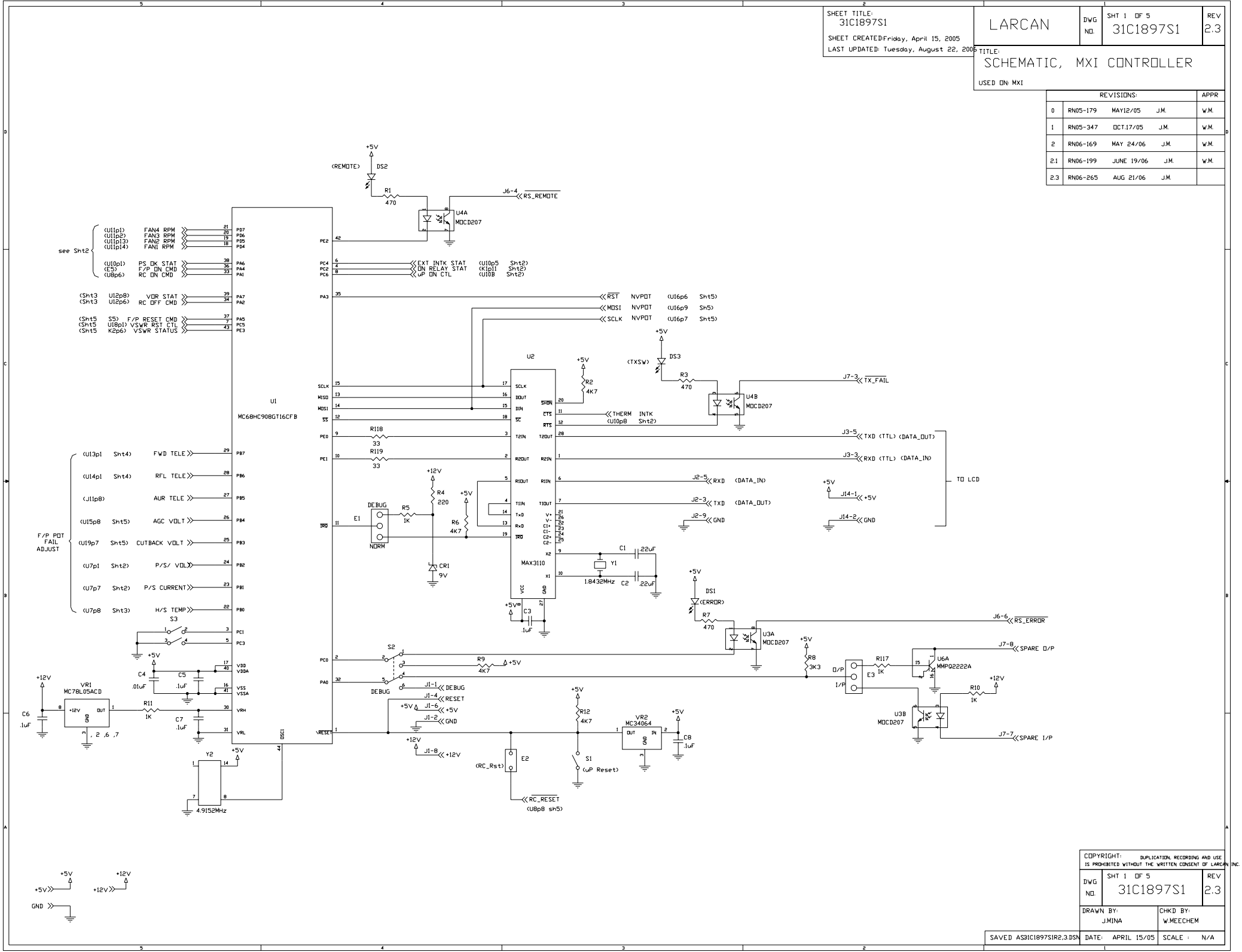
Figure 24 MXi Controller Board Schematic 31C1897S1 sht1 Rev 2.3
