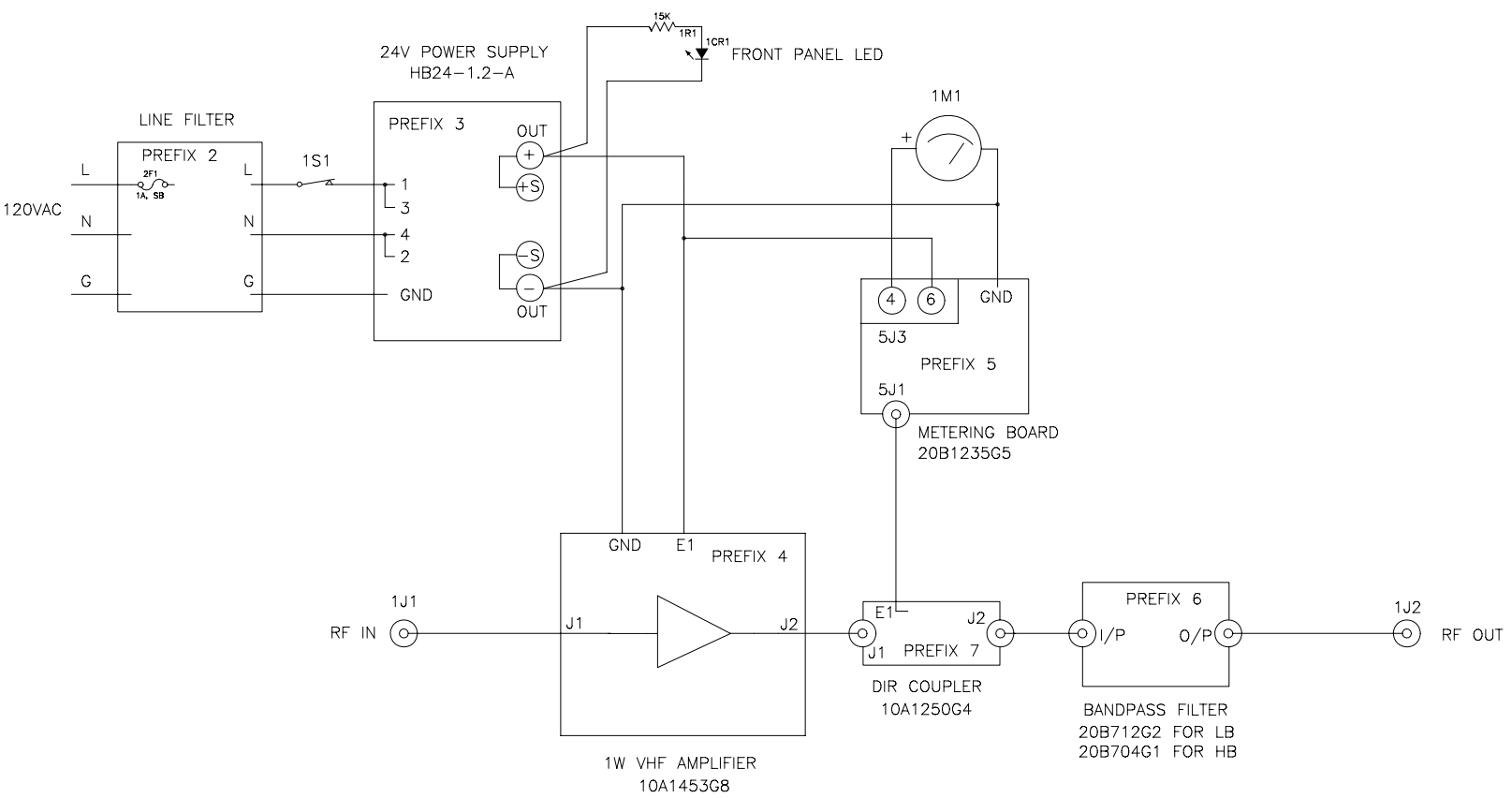
1W VHF AMPLIFIER WIRING & BLOCK DIAGRAM: 20B2449 PUB99-94 rev0: FIGURE 94-2
