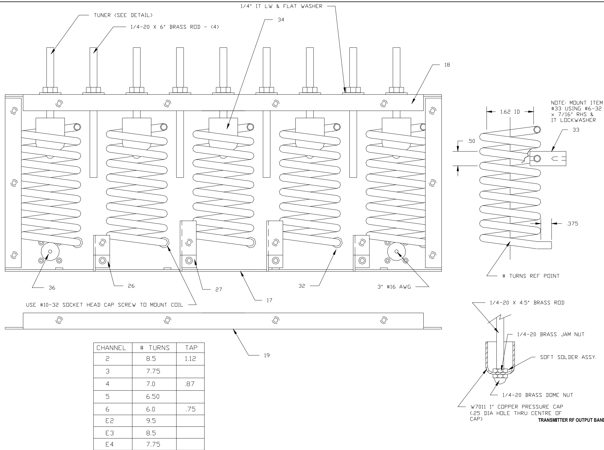
Figure 4 Generic Bandpass Filter Assembly 30C1064 sht2 Rev 3
