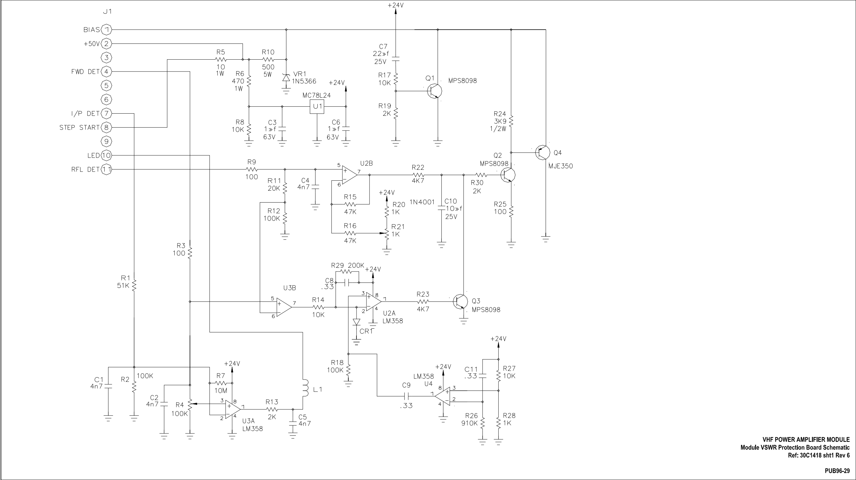
Figure 8 Module VSWR Protection Board Schematic 30C1418 sht 1 rev 6
