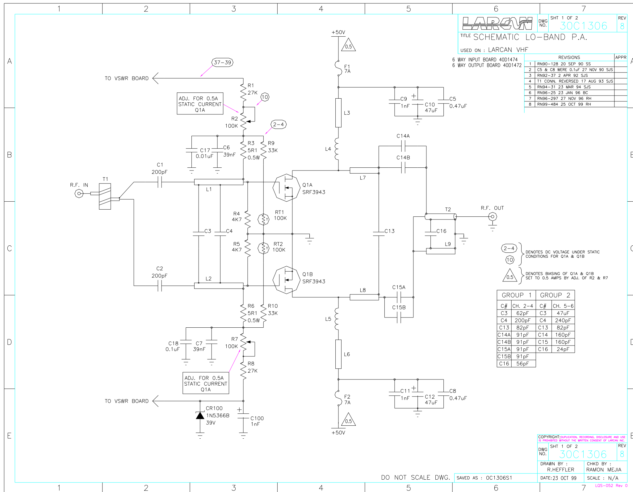
Figure 5 Single Stage PA Schematic 30C1306 sht 1 rev 8
