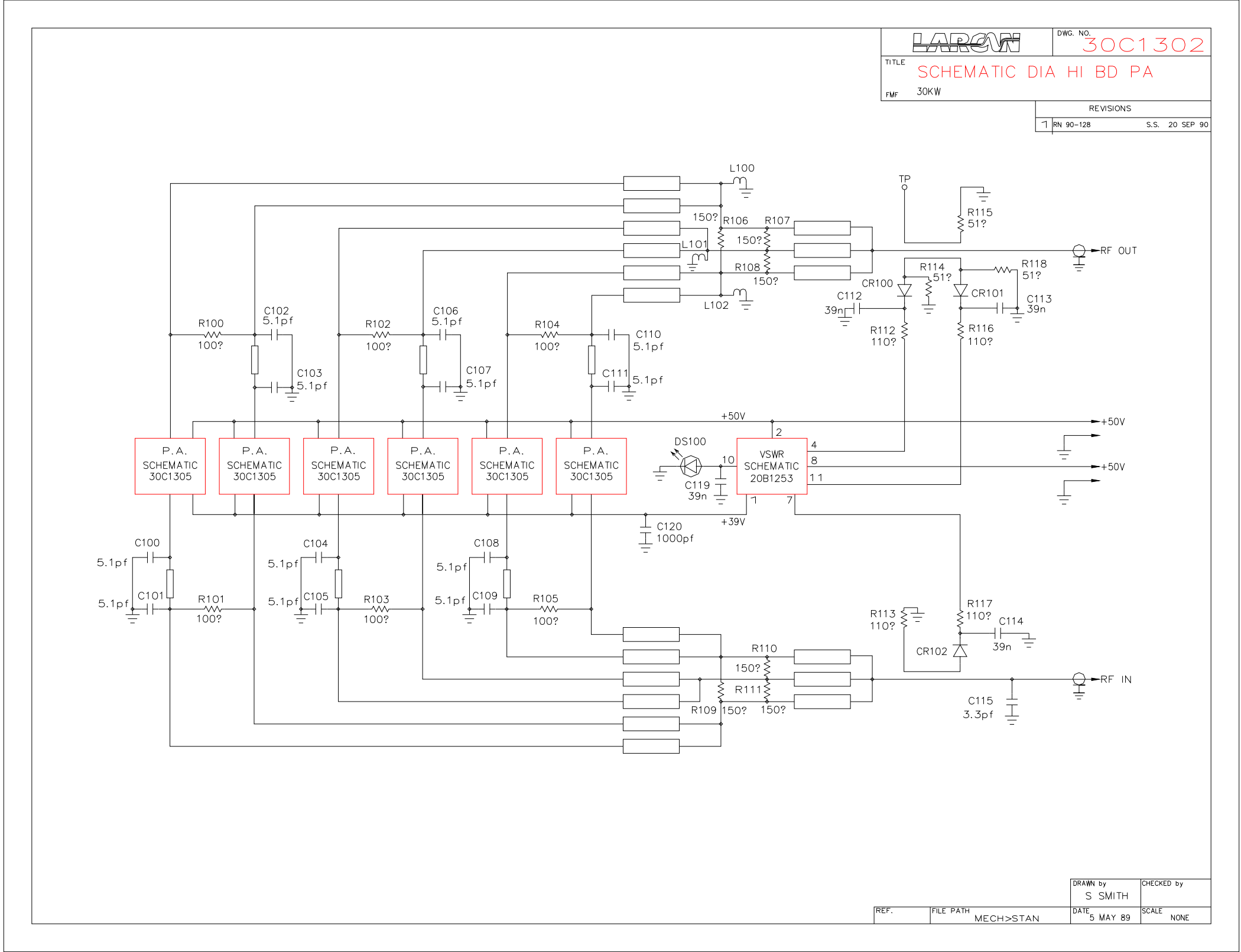
Figure 3 Module Schematic 30C1302 sht1 rev 1
