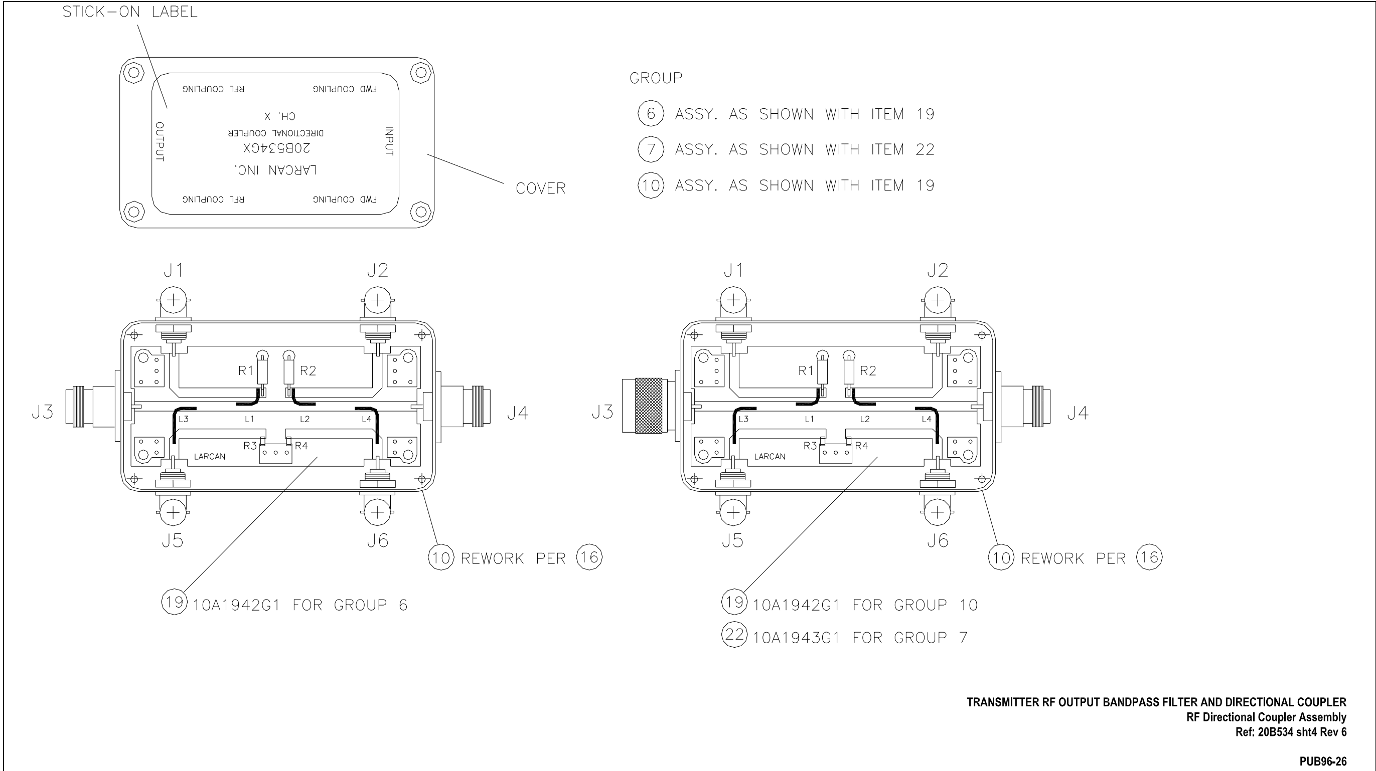
Figure 5 RF Directional Coupler Assembly 20B534 sht4 Rev 6
