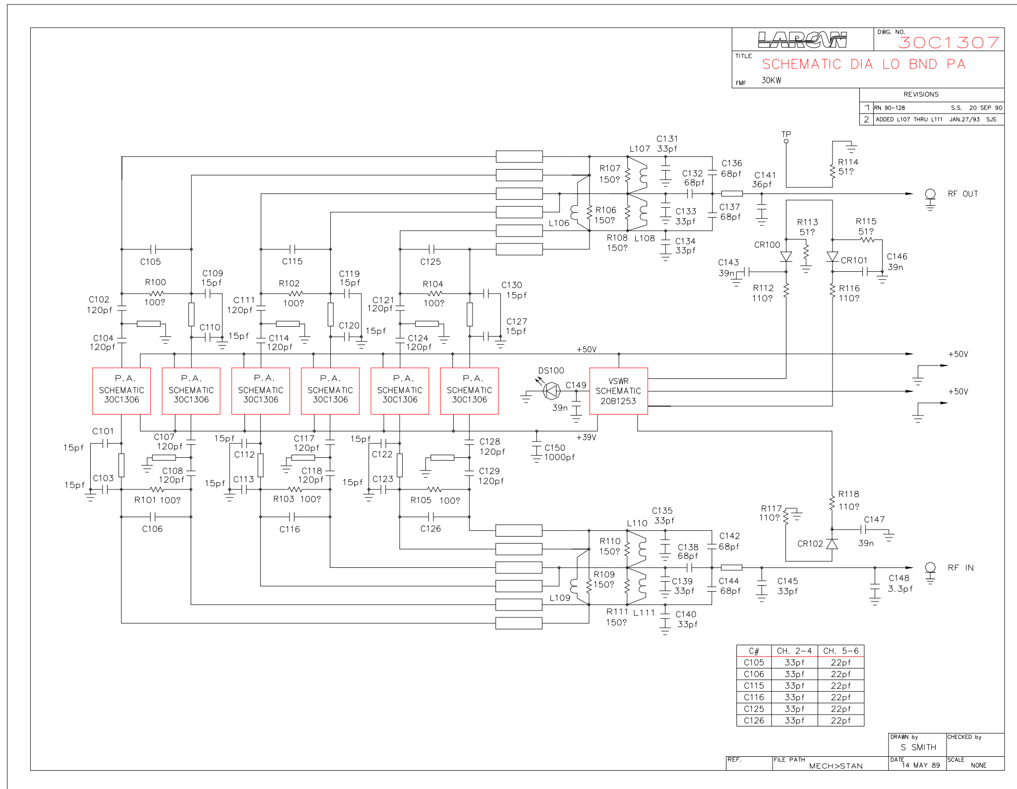
Figure 3 Module Schematic 30C1307 rev 2
