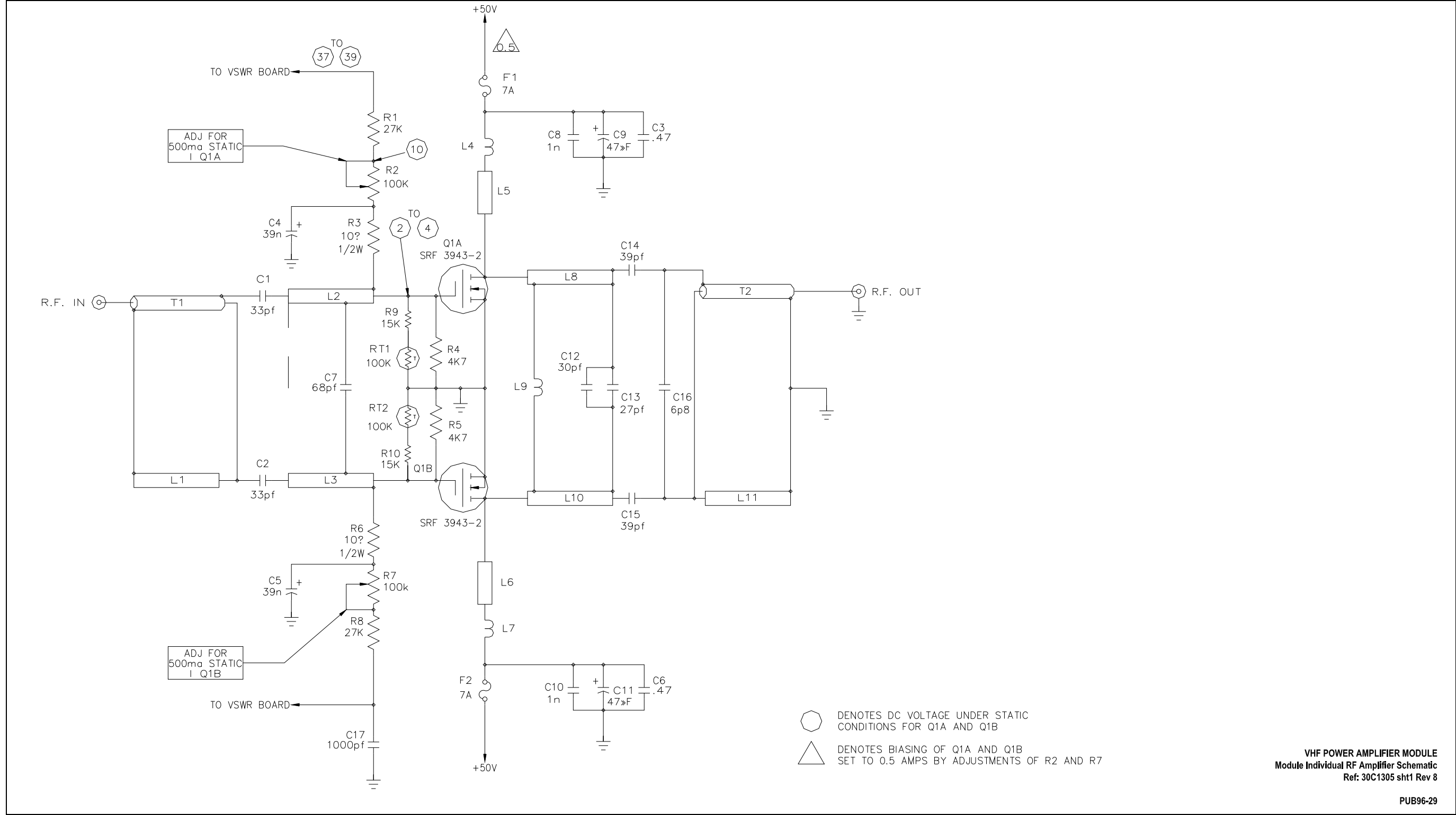
Figure 5 Single Stage PA Schematic 30C1305 sht 1 rev 8
