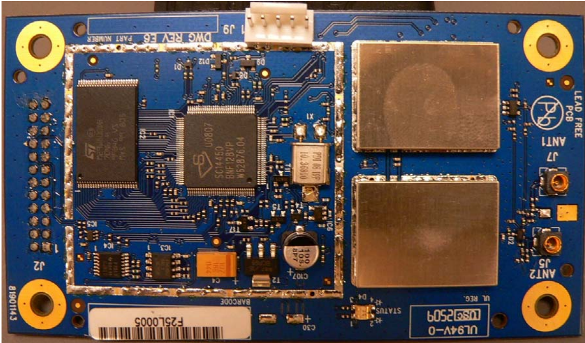
Top view of EUT with RF shield
