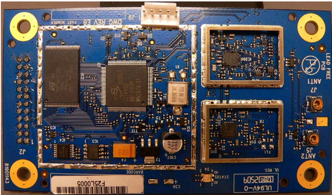
Top view of EUT with RF shield removed
