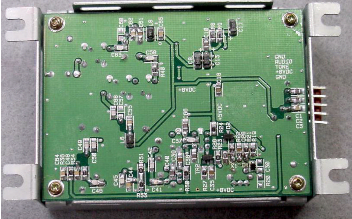
TX MODULE BOTTOM WITHOUT SHIELD FILE: TX MODULE BOTTOM WITHOUT SHIELD.JPG
