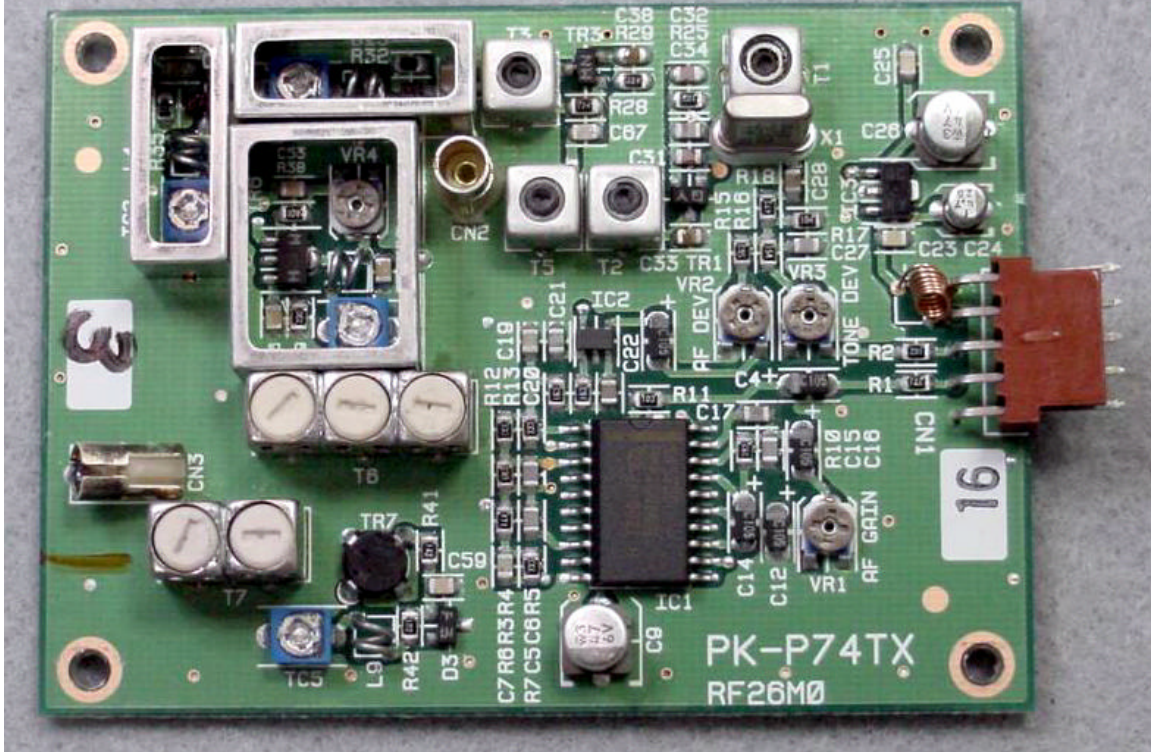
TX MODULE TOP WITHOUT SHIELD FILE: TX MODULE TOP WITHOUT SHIELD.JPG
