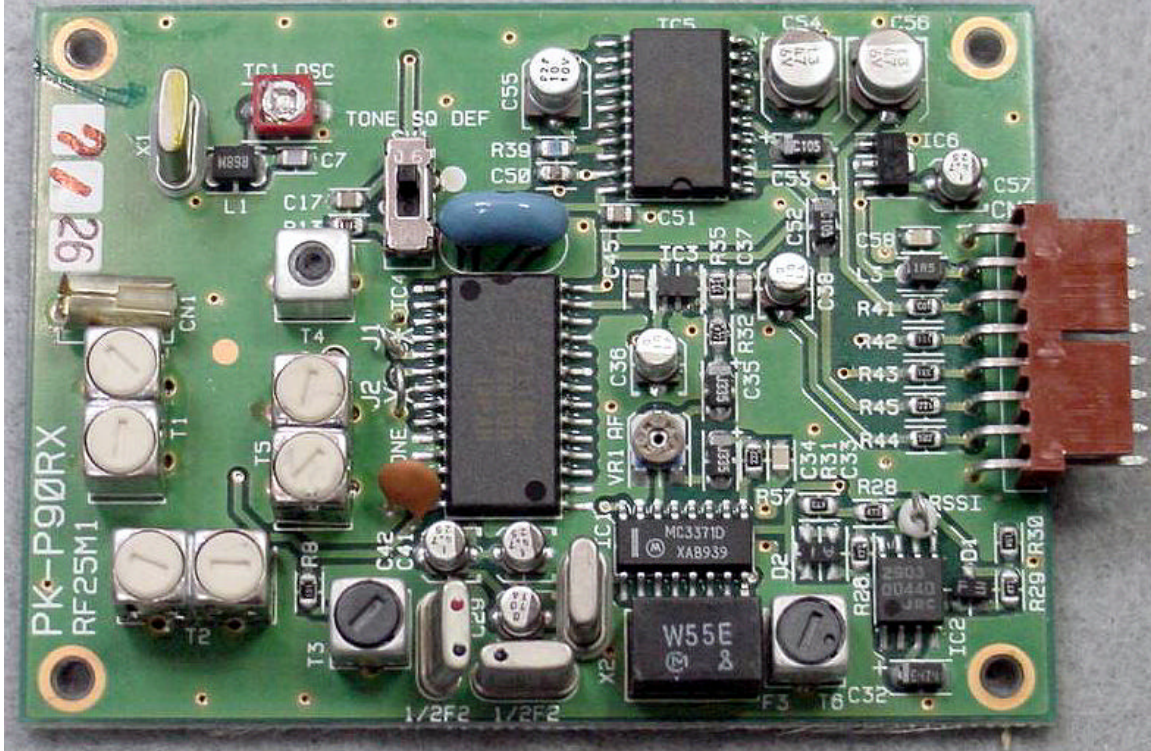
RX MODULE TOP WITHOUT SHIELD FILE: RX MODULE TOP WITHOUT SHIELD.JPG
