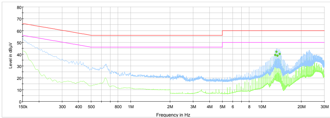
HME Clearcom NEX-350341 CE 120 Vac 60 Hz Phase Preview Result 2-AVG Preview Result 1-PK+ CISPR 32 Mains Q-Peak Class B Limit CISPR 32 Mains Average Class B Limit Final_Result QPK Final_Result CAV
