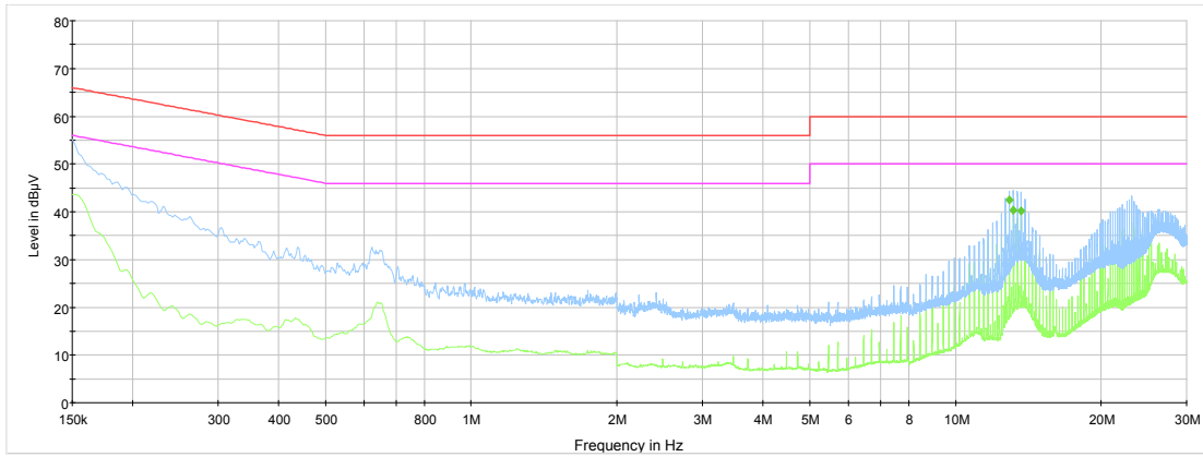
HME Clearcom NEX-350341 CE 120 Vac 60 Hz Neutral Preview Result 2-AVG Preview Result 1-PK+ CISPR 32 Mains Q-Peak Class B Limit CISPR 32 Mains Average Class B Limit Final_Result QPK Final_Result CAV
