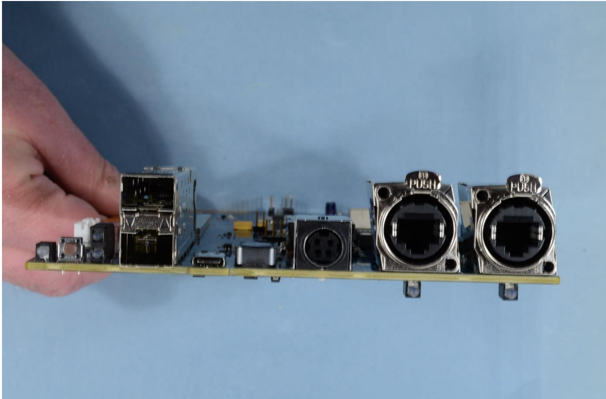
Connectors
