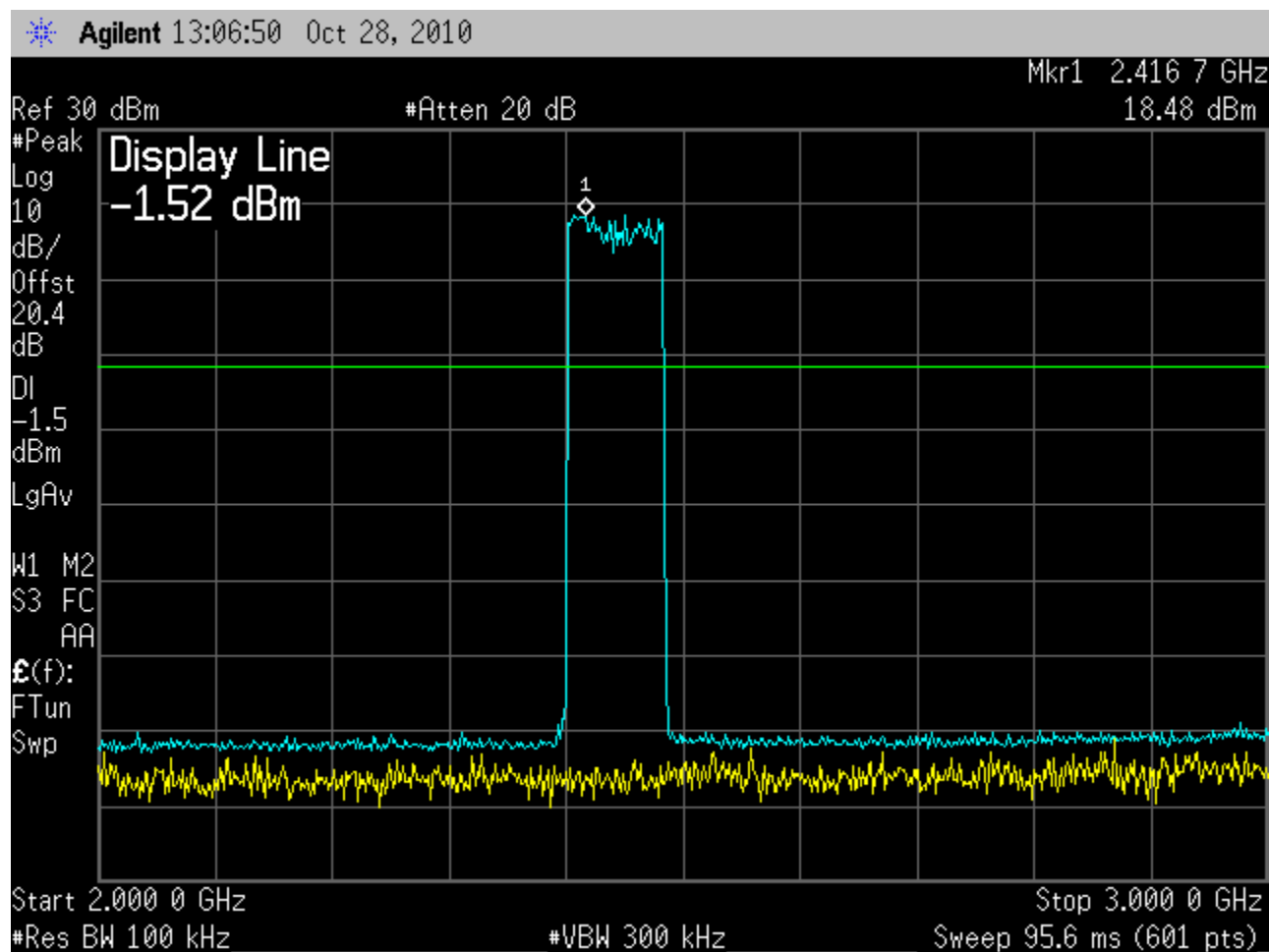
Plots from 2GHz to 3GHz , Display Line -1.52 dBm which is 20dB below the highest in band emission.
