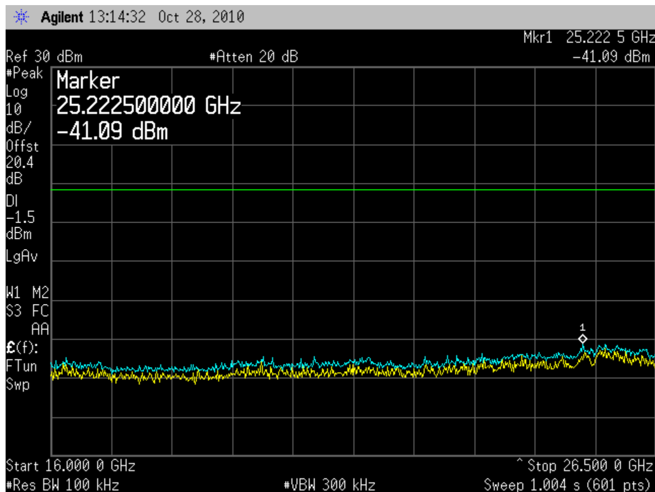
Plots from 16GHz to 26.5GHz , Display Line is -1.52 dBm which is 20dB below the highest in band emission.
