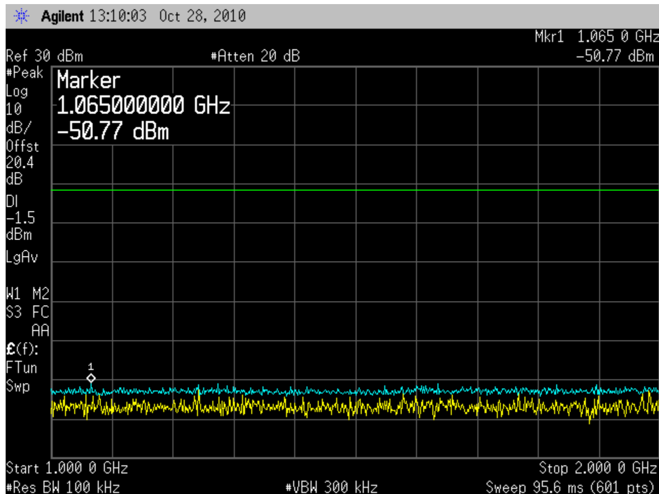
Plots from 1GHz to 2GHz , Display Line is -1.52 dBm which is 20dB below the highest in band emission.
