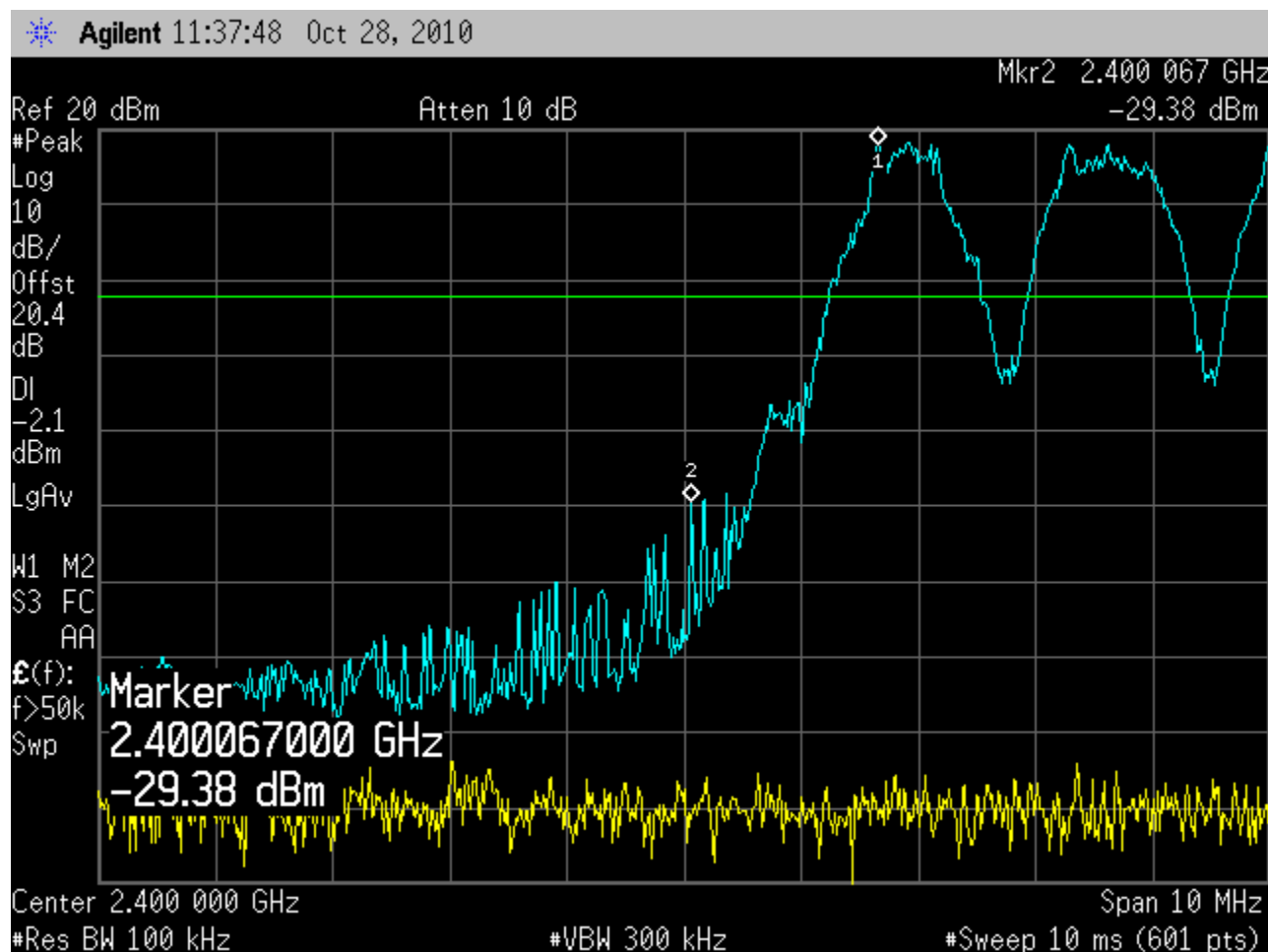
Lower Band edge (Hopping)
