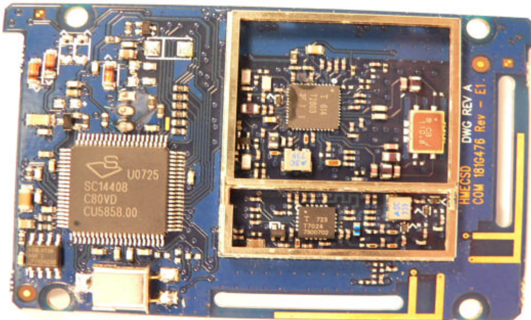
BP200 Board, Top side without shield
