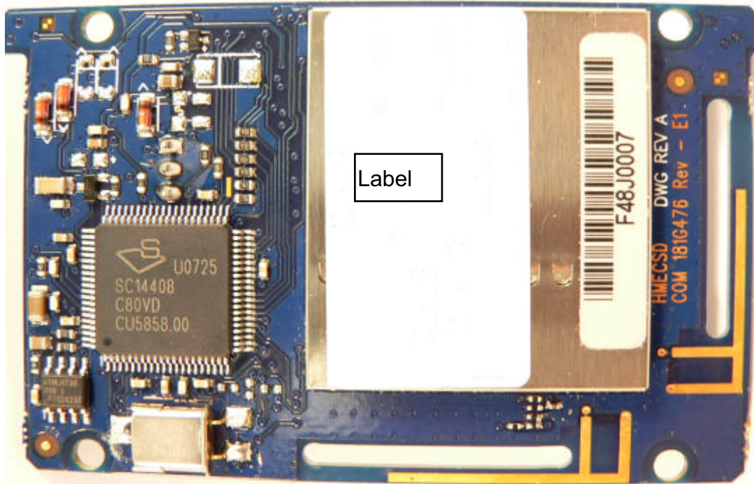
BP200 Board, Top side with shield
