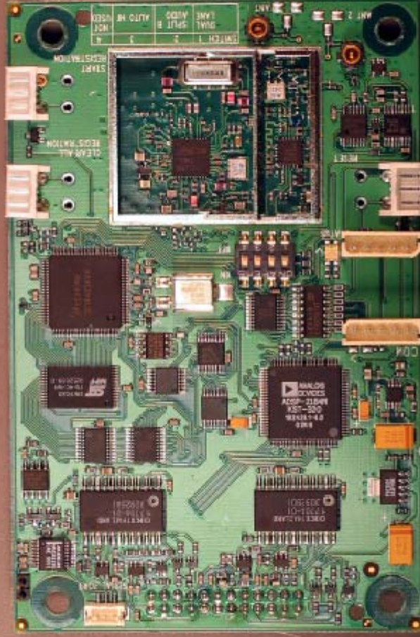
BS200 XCVR Board Top View wo/Shield
