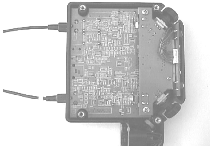
MAIN PCB (BACK) - INTERNAL
