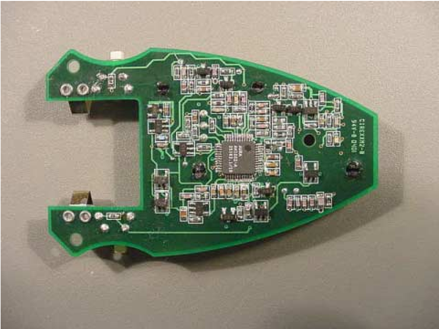
PCB SIDE OPPOSITE ANTENNAS
