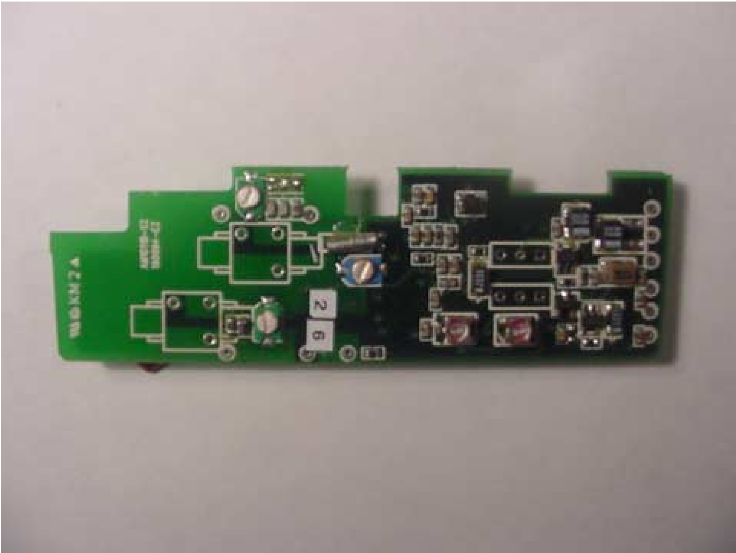
COM XCVR BOARD ANTENNA SIDE 1 WITHOUT FILTERS
