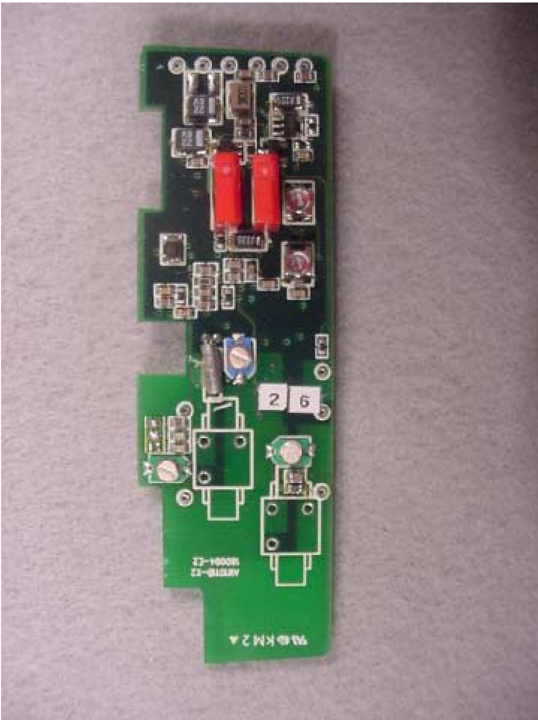
VIEW OF PCB WITH ANTENNAS REMOVED
