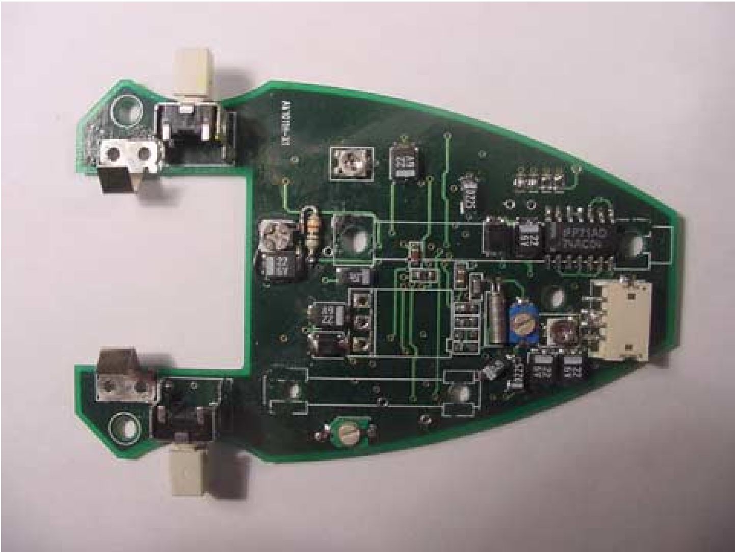
PCB VIEW WITH ANTENNAS AND CERAMIC FILTERS REMOVED
