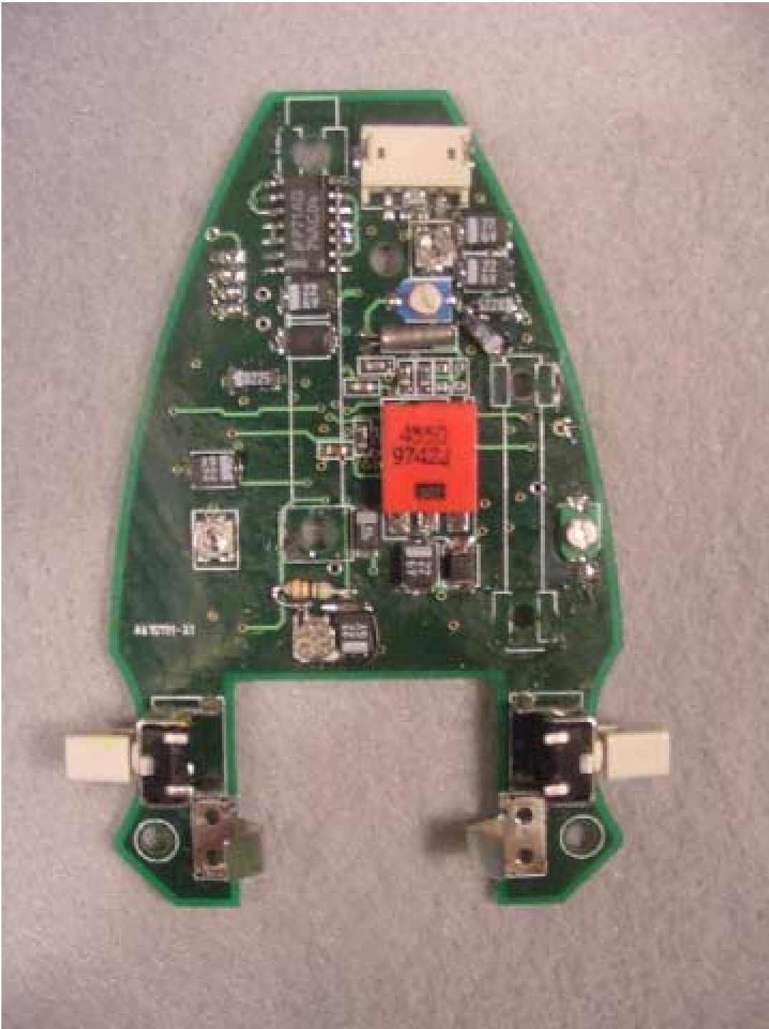
PCB VIEW WITH ANTENNAS REMOVED
