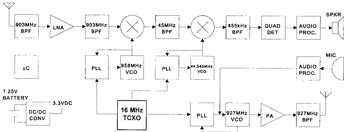
Figure 1 Block Diagram of COM900CC
