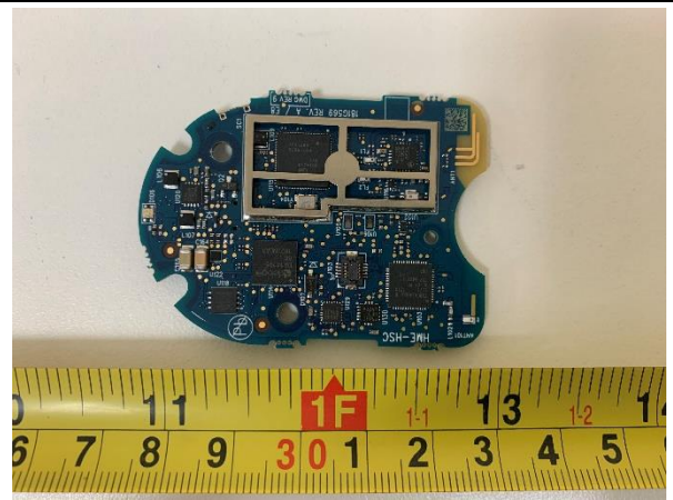
Internal - Main PCBA Top
