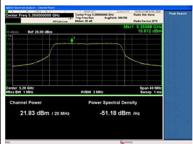
5260MHz-PWR
