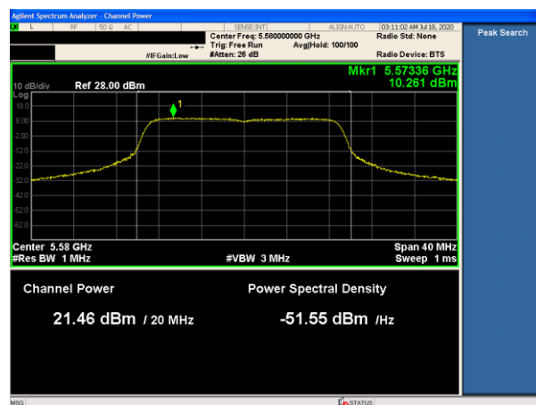
5580MHz-PWR
