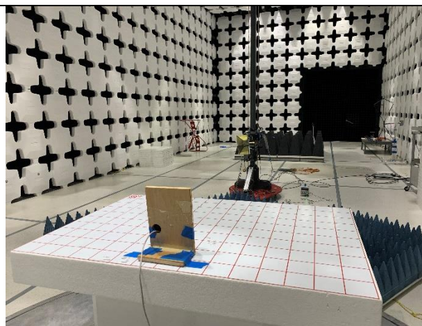
RE Above 1GHz – Rear View
