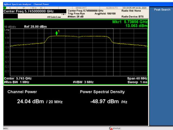
5745MHz-PWR
