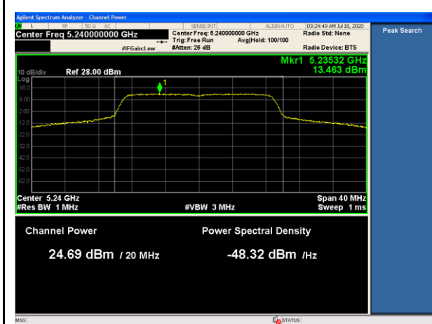
5240MHz-PWR
