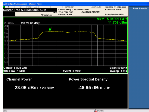
5825MHz-PWR
