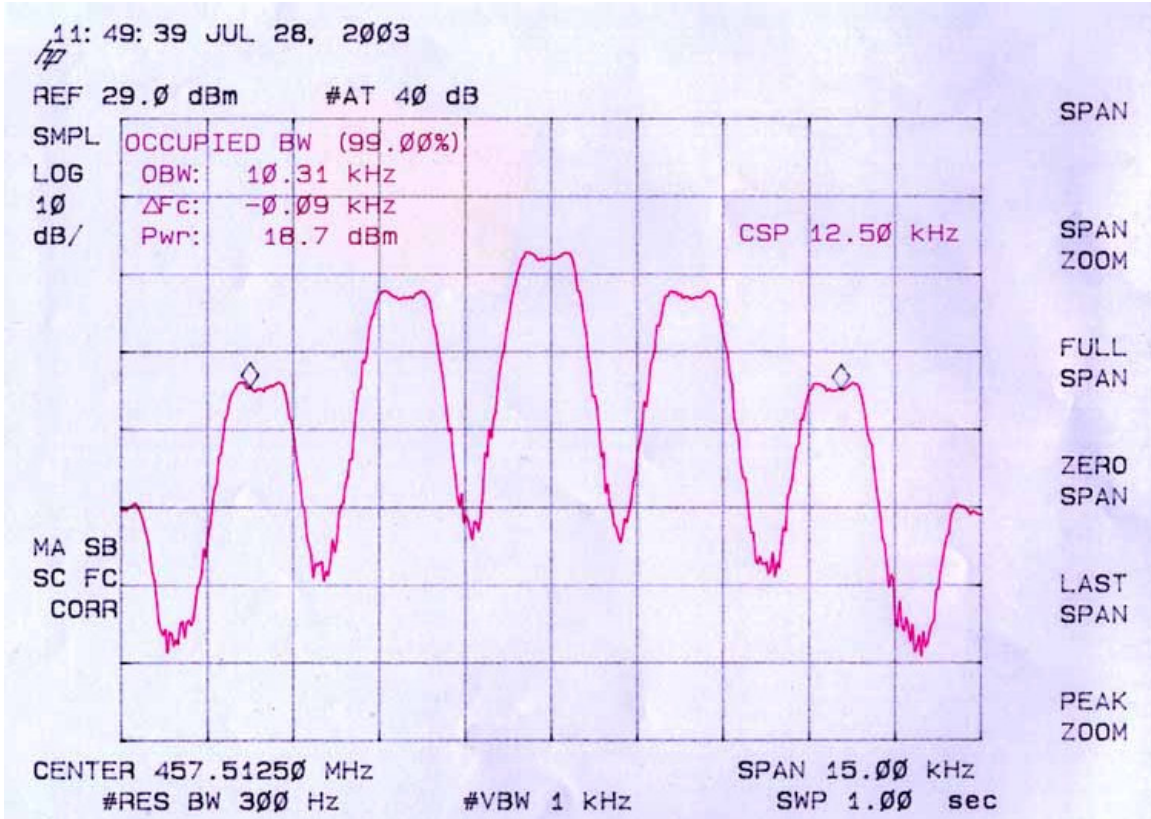
Figure 1 BASE 400 Modulated with 2500Hz + 16dB
