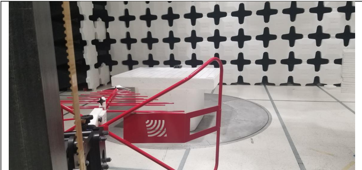
Radiated Emission Test below 1GHz Front View
