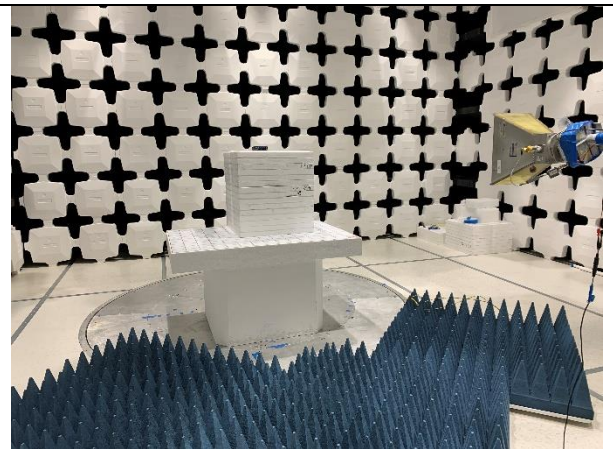
RE Below 1GHz – Rear View
