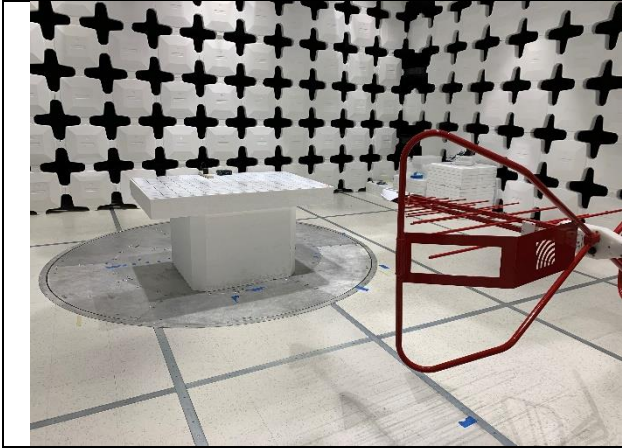
RE Below 1GHz – Front View
