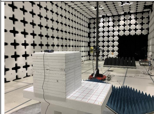
RE Above 1GHz – Front View
