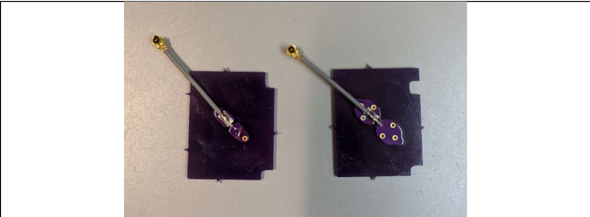
5GHZ ANTENNA BOARD – TOP VIEW
