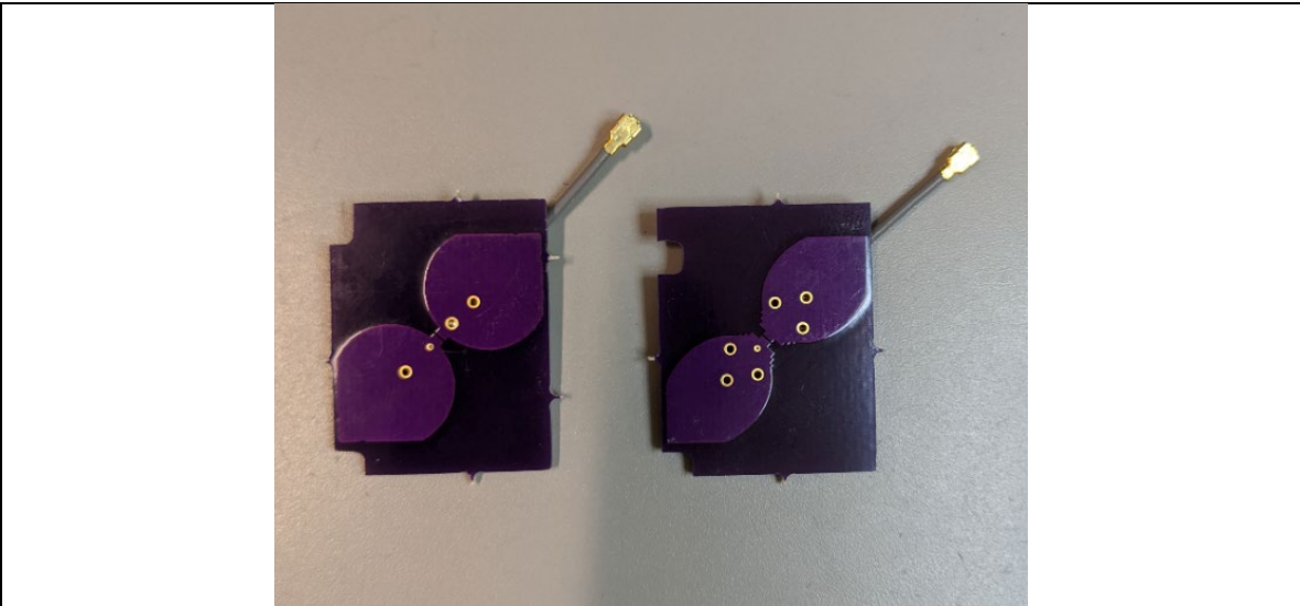
5GHZ ANTENNA BOARD – BOTTOM VIEW
