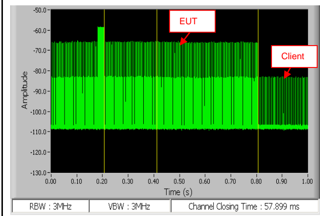
Channel Closing Time – 5300MHz (Type0)
