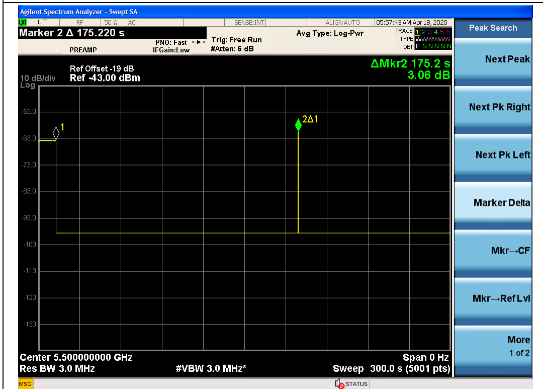
Radar at beginning of CAC -5500MHz
