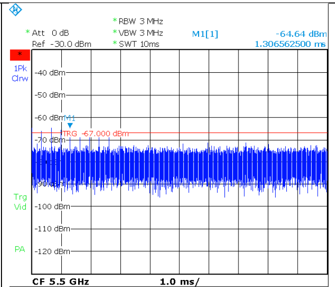
Radar Type 6 @ 5500MHz
