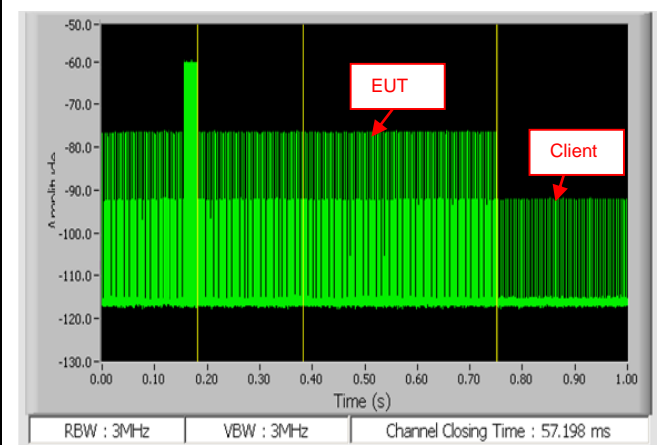
Channel Closing Time – 5500MHz (Type0)
