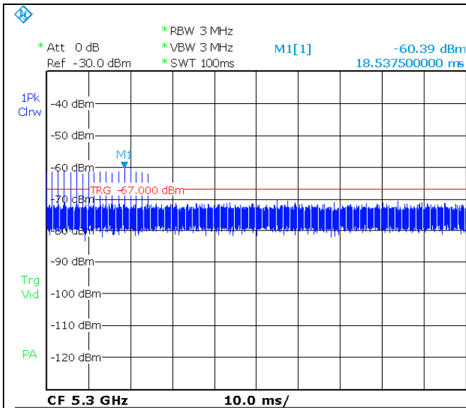
Radar Type 0 @ 5300MHz
