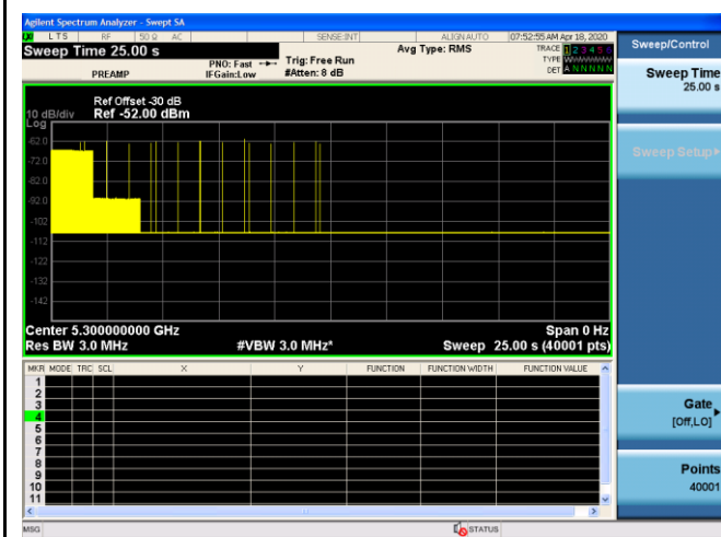
Channel Move Time& Closing Time – 5300MHz (Type5)
