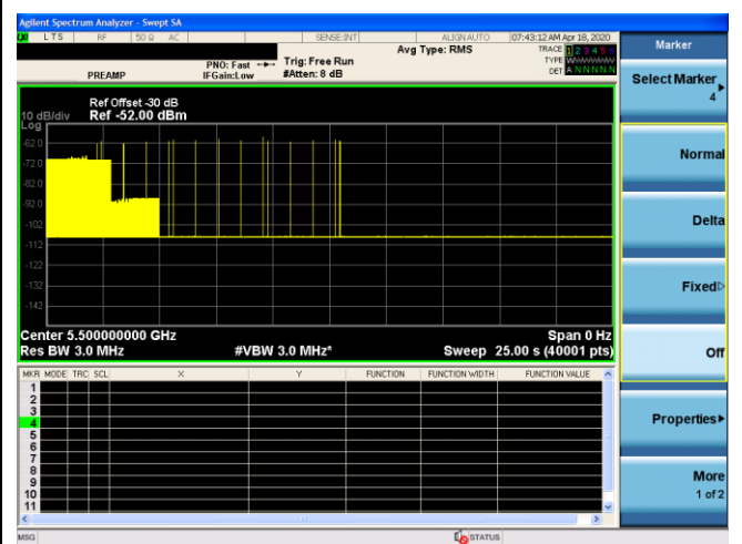
Channel Move Time& Closing Time – 5500MHz (Type5)
