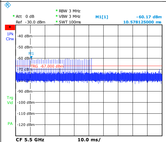
Radar Type 0 @ 5500MHz
