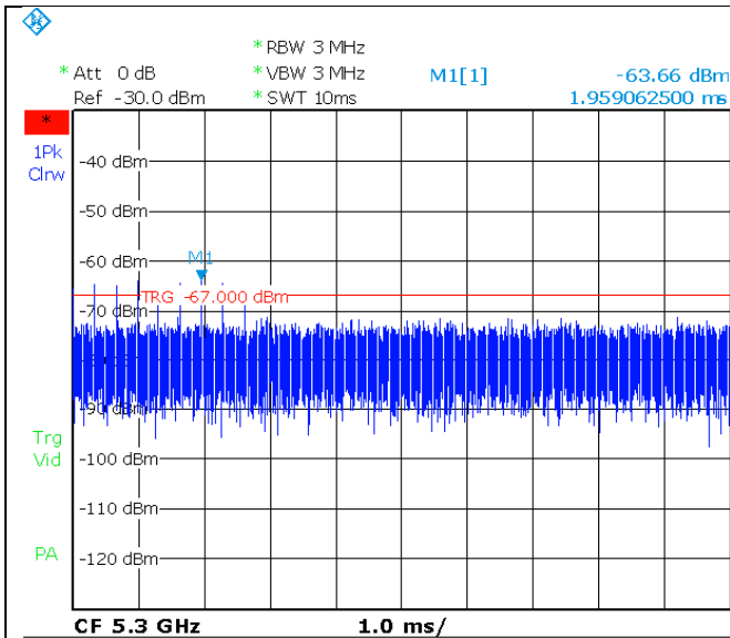
Radar Type 6 @ 5300MHz
