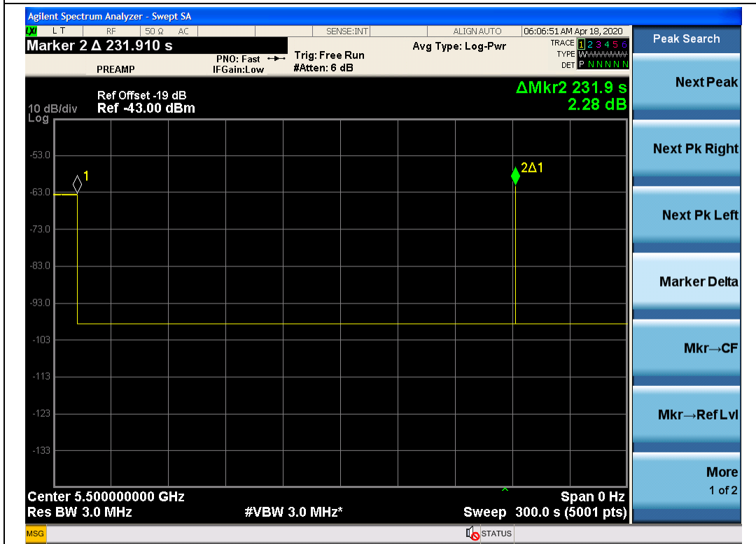
Radar at end of CAC -5500MHz
