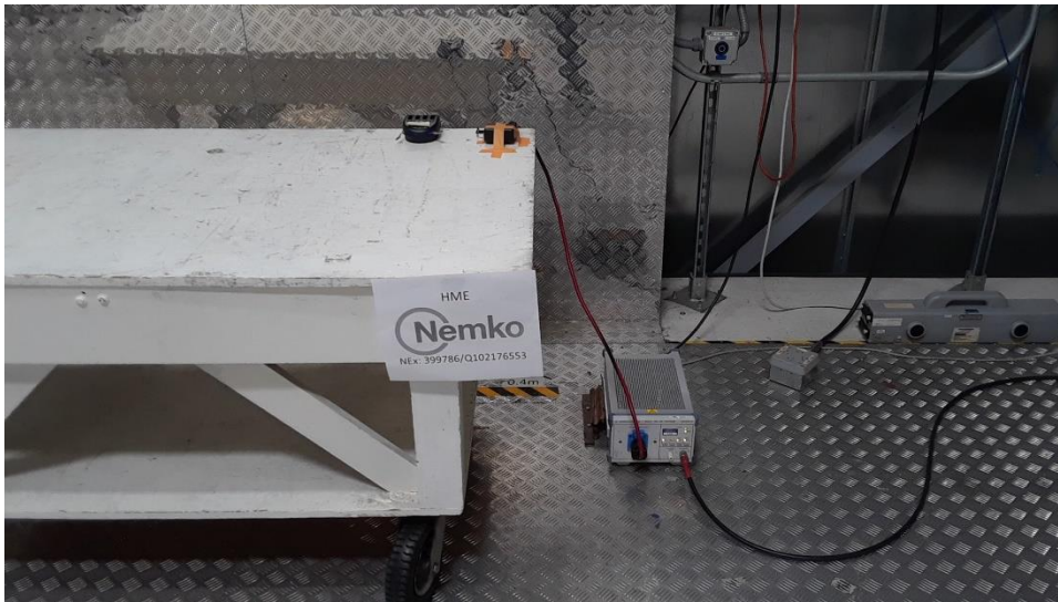
Figure 5 - Conducted AC emissions, front view
