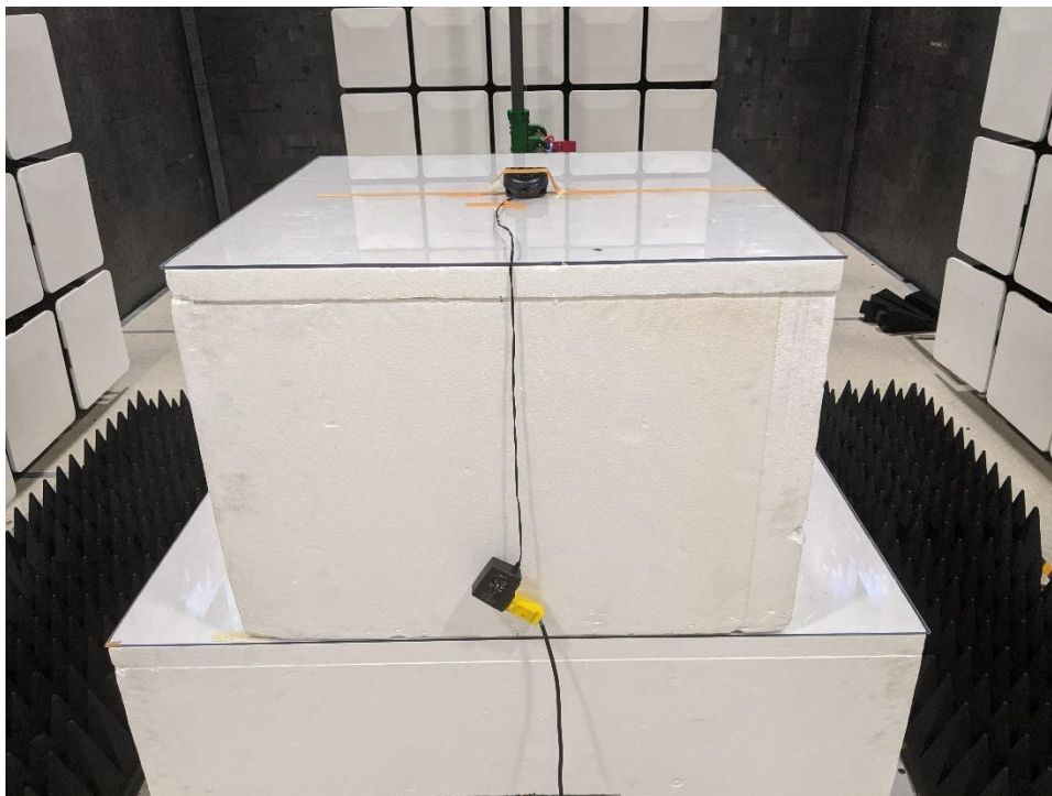
Figure 4 - Radiated emissions above 1 GHz, back view
