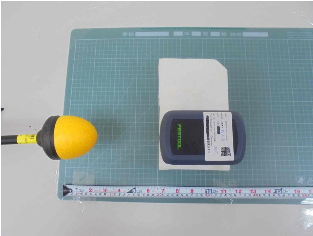
E-Field (Standby Mode - Bottom_20cm)
