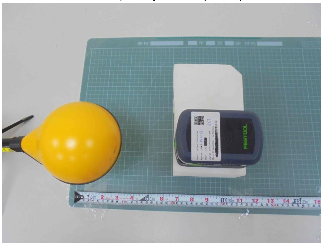
H-Field (Standby Mode - Top_20cm)
