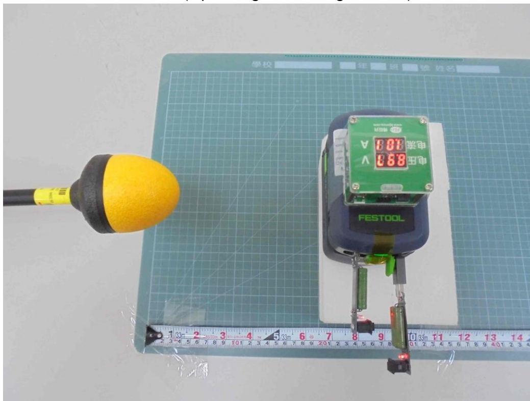
E-Field (Operating Mode - Right_20cm)
