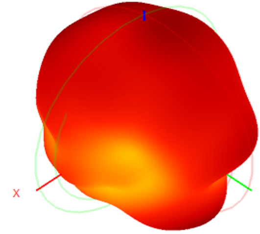
2420.0MHz H+V, Eff: 24.4%
