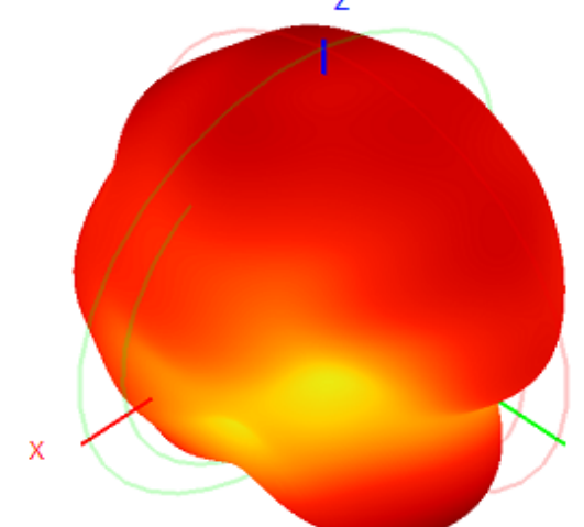
2470.0MHz H+V, Eff: 27.6%
