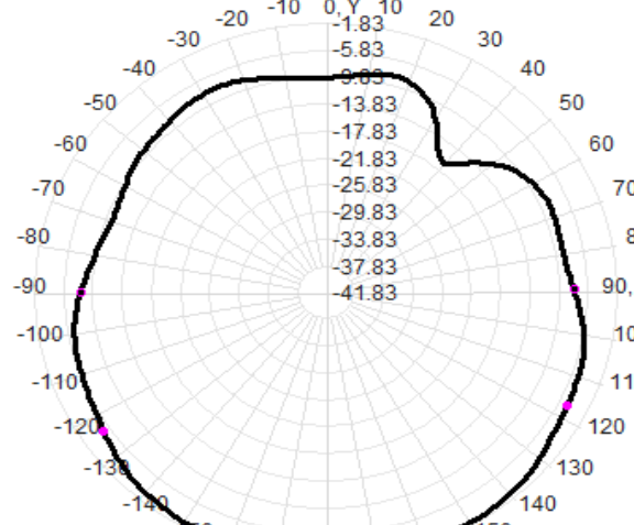
Total(H-XY), Max=-2.05dBi, CirD=14.72
