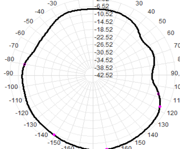
Total(H-XY), Max=-3.15dBi, CirD=10.94
