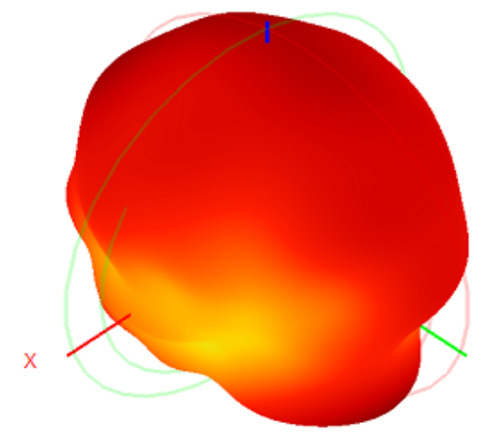
2430.0MHz H+V, Eff: 23.9%
