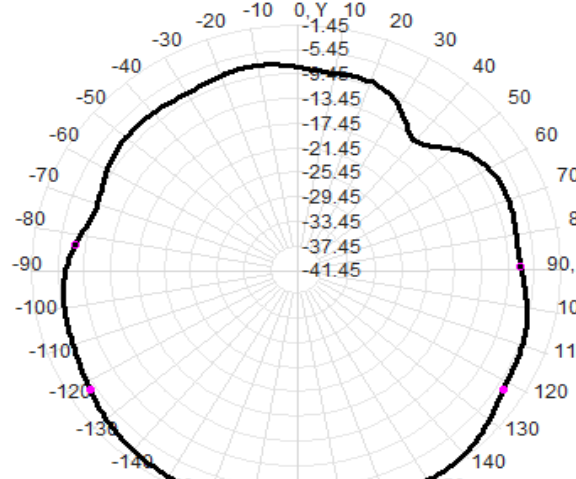
Total(H-XY), Max=-2.01dBi, CirD=10.10
