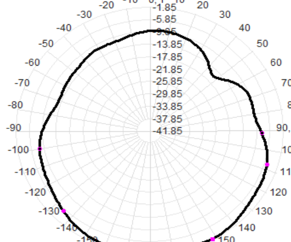
Total(H-XY), Max=-2.37dBi, CirD=15.24
