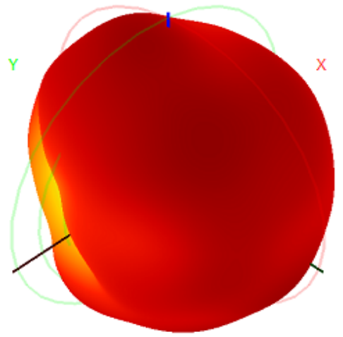
2400.0MHz H+V, Eff: 24.5%
