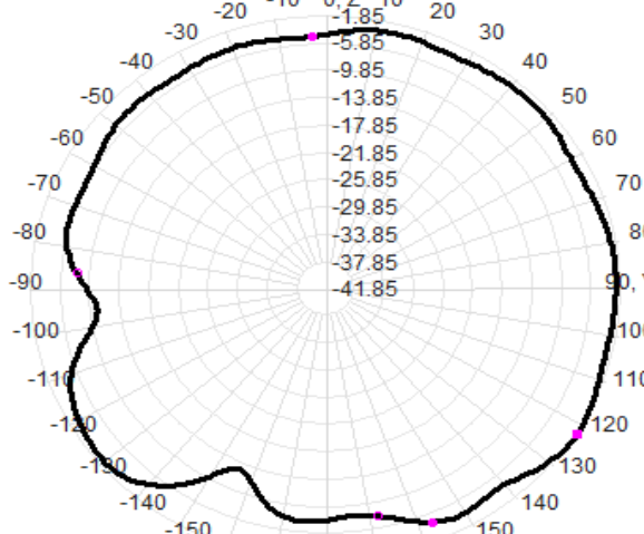
2470.0MHz Total(E2-YZ), Max=-1.83dBi
