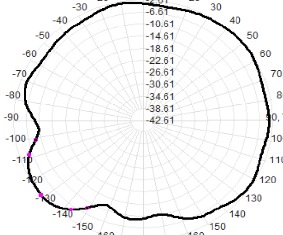
2420.0MHz Total(E2-YZ), Max=-2.25dBi
