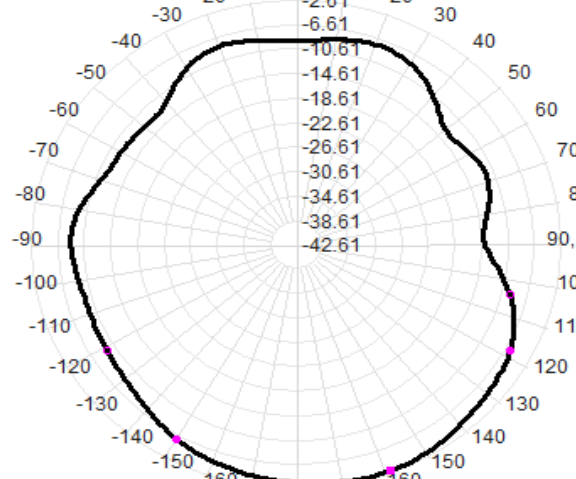
Total(H-XY), Max=-2.70dBi, CirD=11.56
