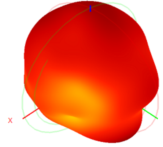
2400.0MHz H+V, Eff: 24.5%
