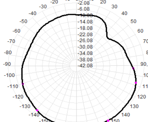
Total(H-XY), Max=-2.55dBi, CirD=13.99
