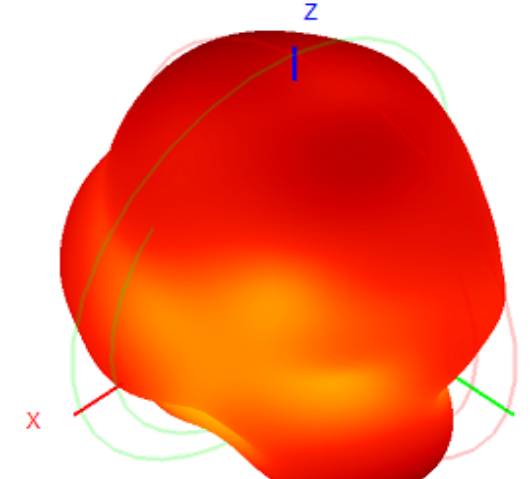
2500.0MHz H+V, Eff: 33.5%
