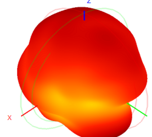
2480.0MHz H+V, Eff: 28.8%
