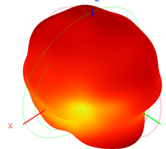
2450.0MHz H+V, Eff: 25.5%
