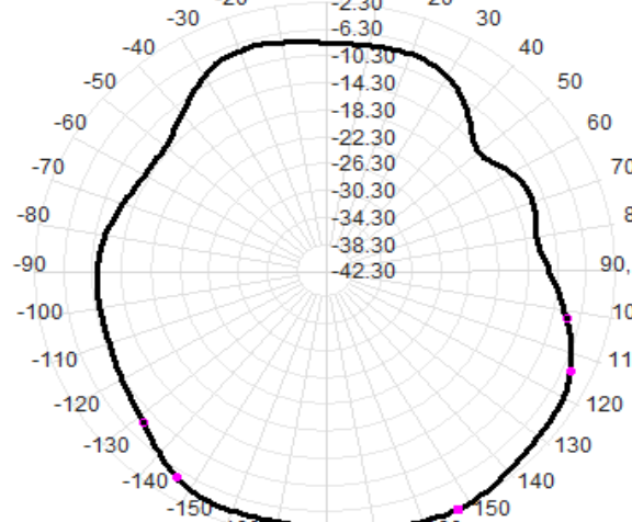
Total(H-XY), Max=-2.53dBi, CirD=12.29
