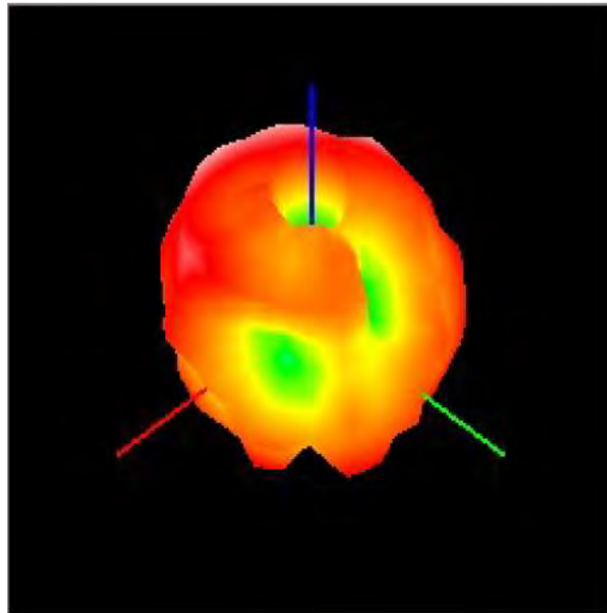
frequency range: 5GHz
