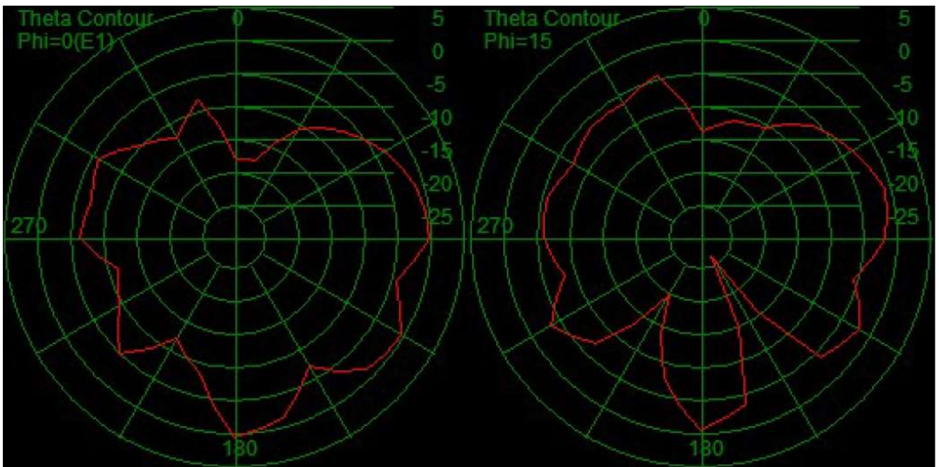
2.4G pattern
