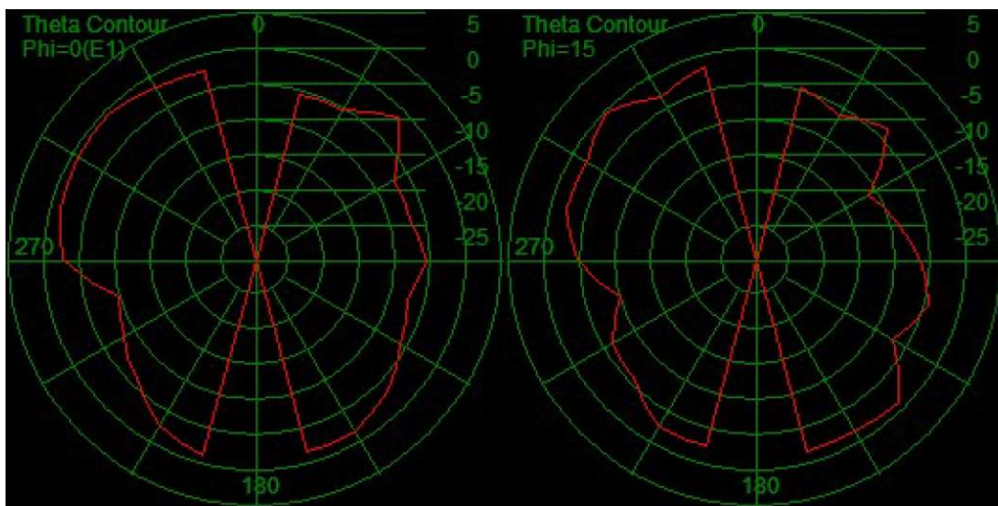
5G pattern
