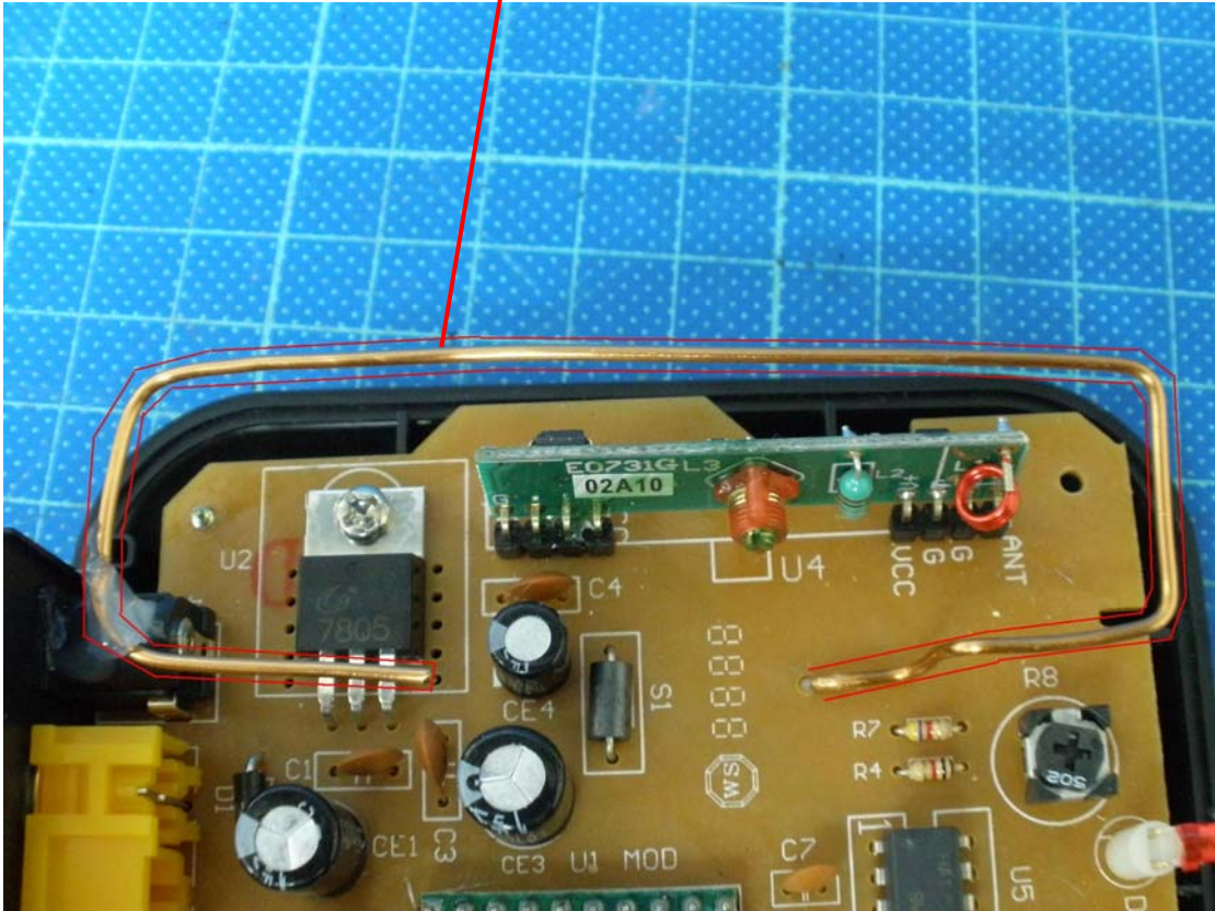
Antenna for 433 MHz
