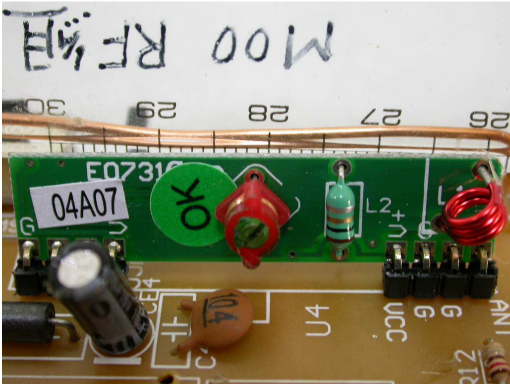
15. Front view of PCB4
