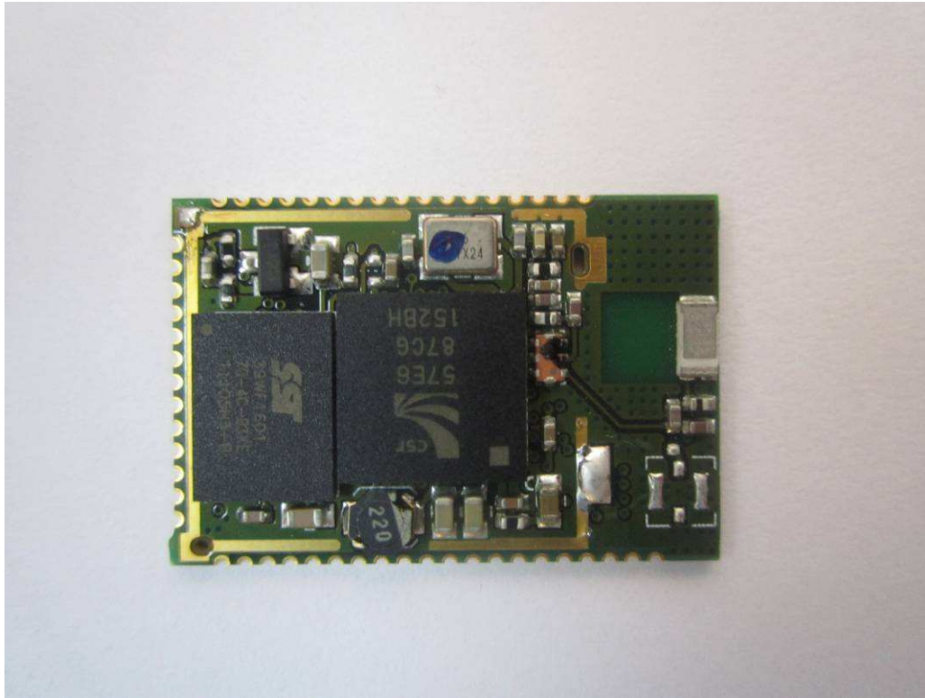
Fig. 5: Internal view
