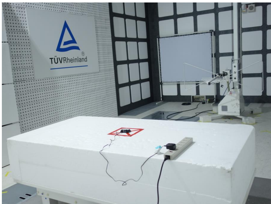
Photograph 10: Set-up for Spurious Emissions (Back View 1)
