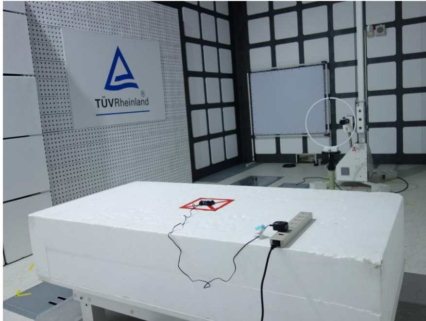
Photograph 11: Set-up for Spurious Emissions (Back View 2)
