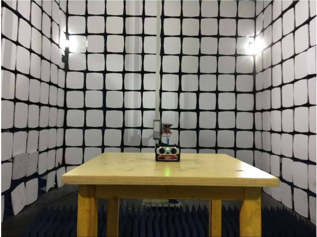
Radiated Emission Test Setup (above 1 GHz) from 1.5M-Height Turntable Test Table
