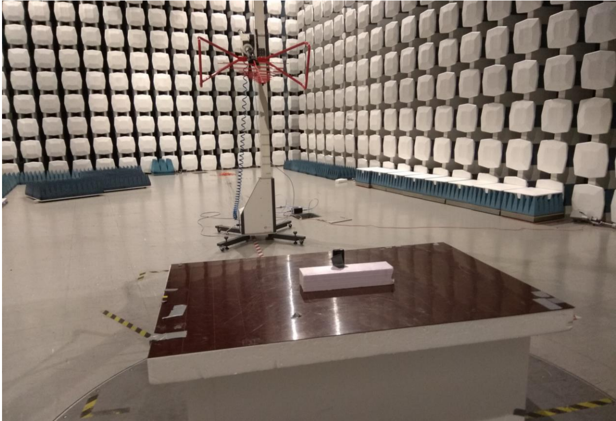
Radiated Emission, Below 1 GHz
