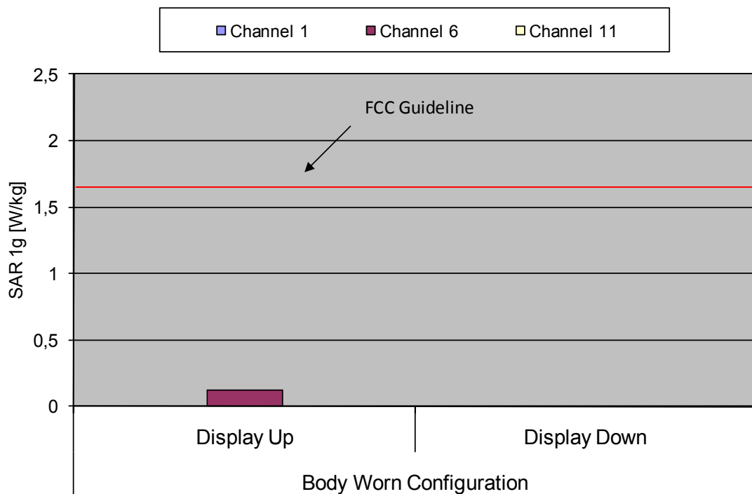
Fig. 11: The measured body SAR values for IEEE 802.11 n (2.45 GHz range) for the Ascom WH1-EACA/PF in body worn configuration, in comparison to the FCC exposure limit.
