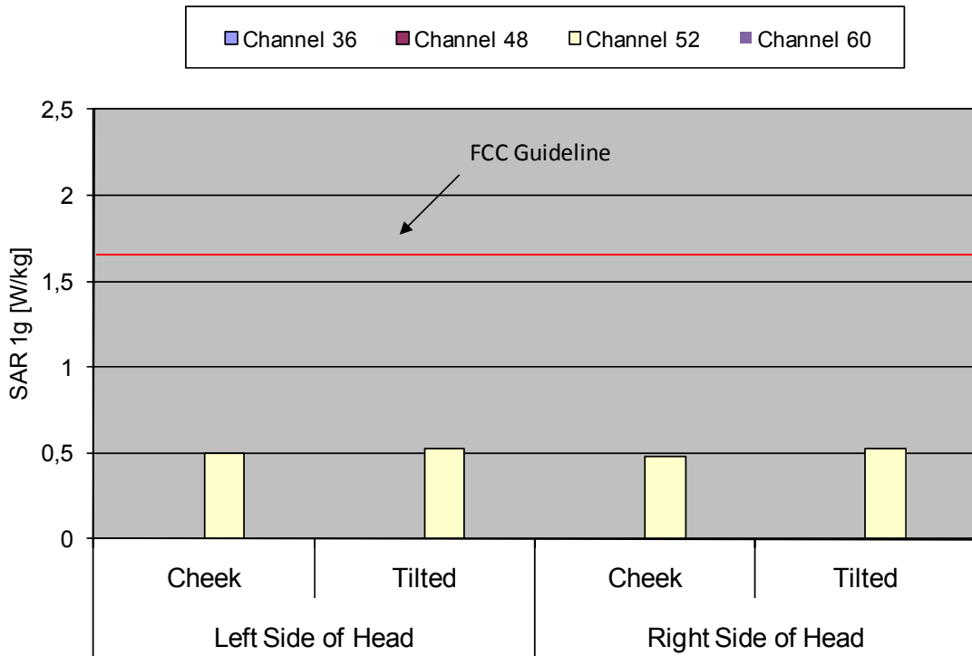
Fig. 12: The measured head SAR values for IEEE 802.11 a (5.2 GHz range) for the Ascom WH1-EACA/PF in head configuration, in comparison to the FCC exposure limit.
