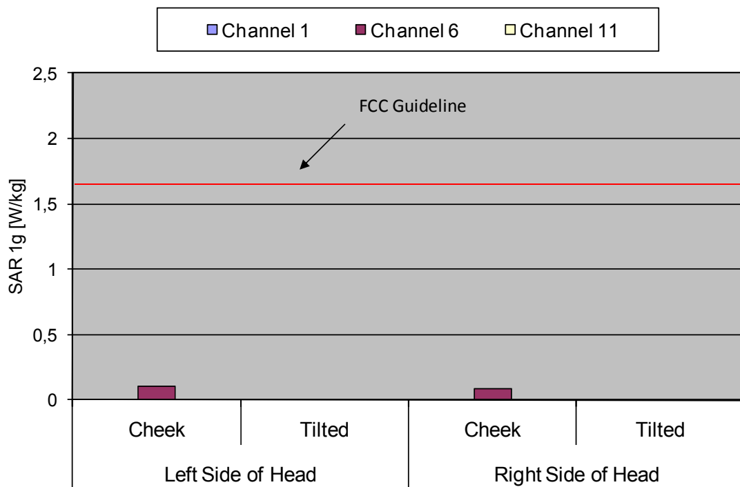
Fig. 9: The measured head SAR values for IEEE 802.11 n (2.45 GHz range) for the Ascom WH1-EACA/PF in head configuration, in comparison to the FCC exposure limit.
