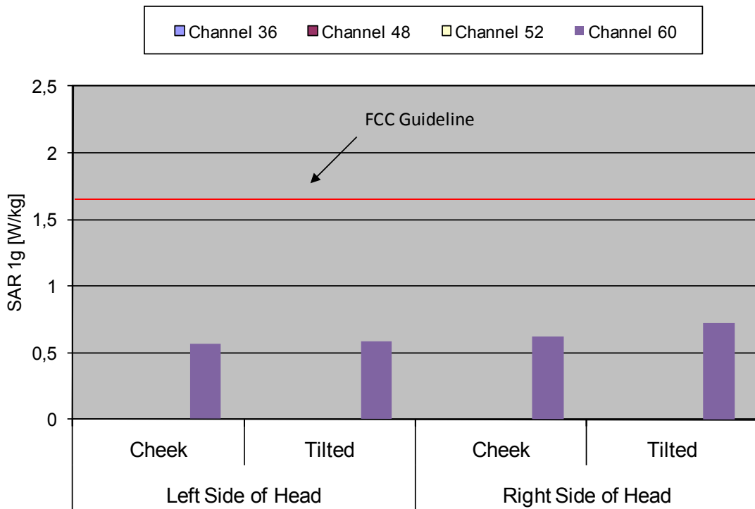
Fig. 13: The measured head SAR values for IEEE 802.11 n (5.2 GHz range) for the Ascom WH1-EACA/PF in head configuration, in comparison to the FCC exposure limit.
