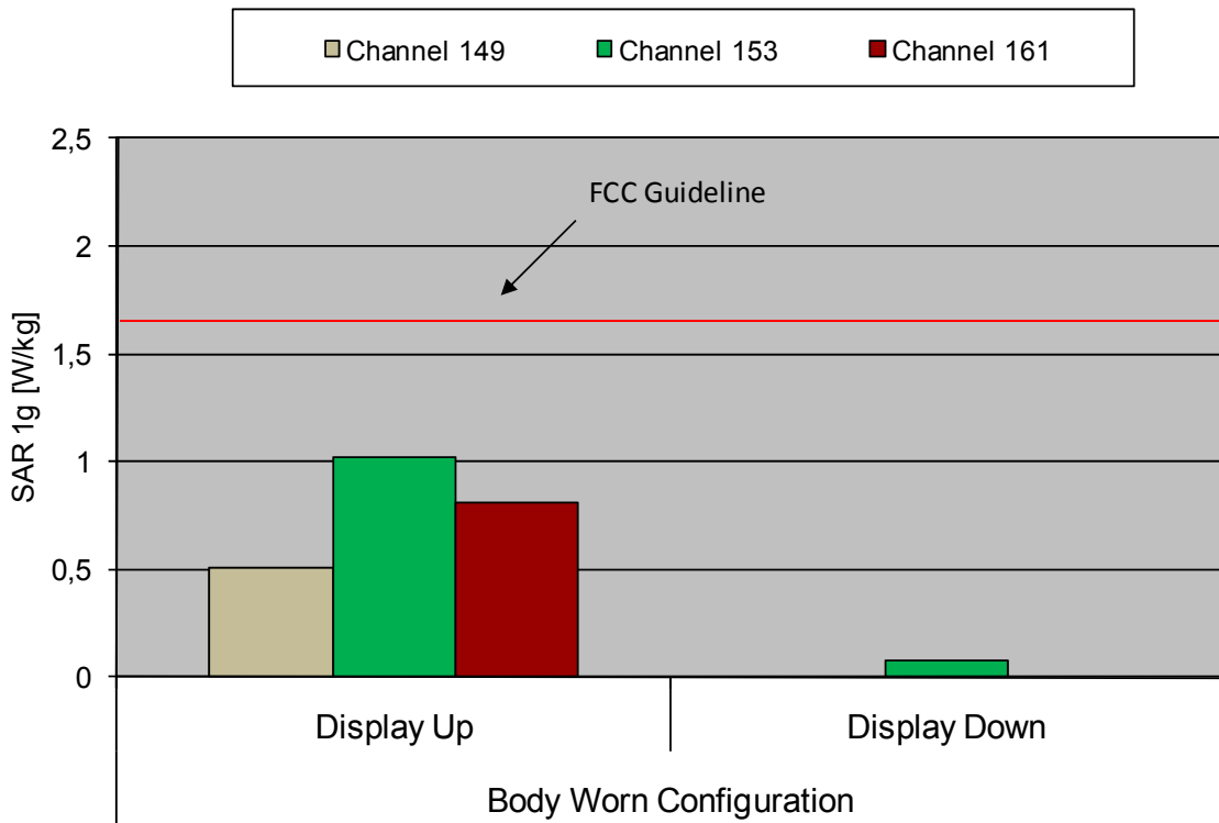
Fig. 23: The measured body SAR values for IEEE 802.11 n (5.8 GHz range) for the Ascom WH1-EACA/PF in body worn configuration, in comparison to the FCC exposure limit.
