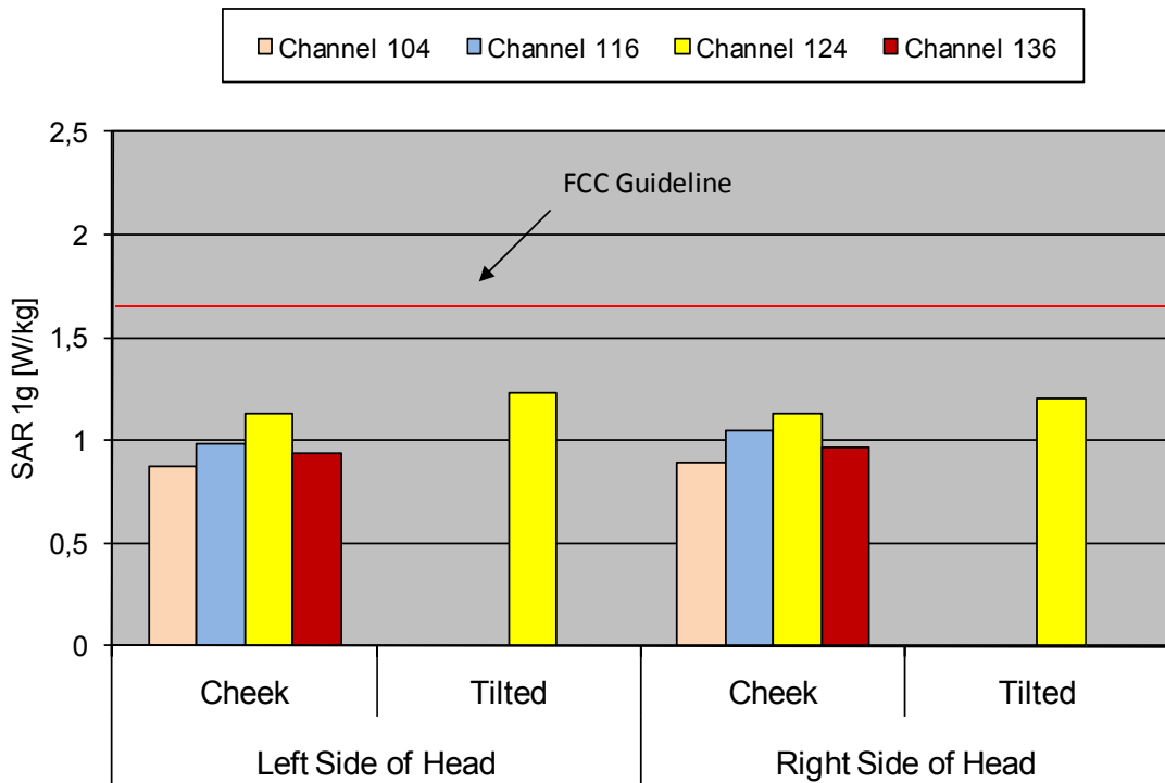
Fig. 17: The measured head SAR values for IEEE 802.11 n (5.5 GHz range) for the Ascom WH1-EACA/PF in head configuration, in comparison to the FCC exposure limit.
