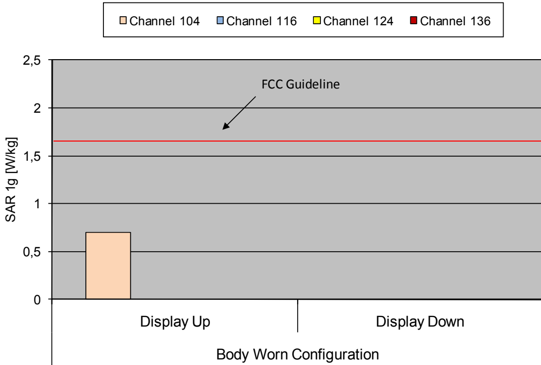
Fig. 18: The measured body SAR values for IEEE 802.11 a (5.5 GHz range) for the Ascom WH1-EACA/PF in body worn configuration, in comparison to the FCC exposure limit.
