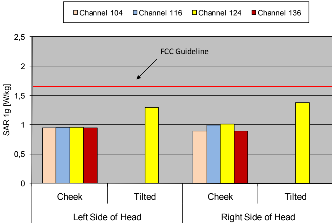
Fig. 16: The measured head SAR values for IEEE 802.11 a (5.5 GHz range) for the Ascom WH1-EACA/PF in head configuration, in comparison to the FCC exposure limit.
