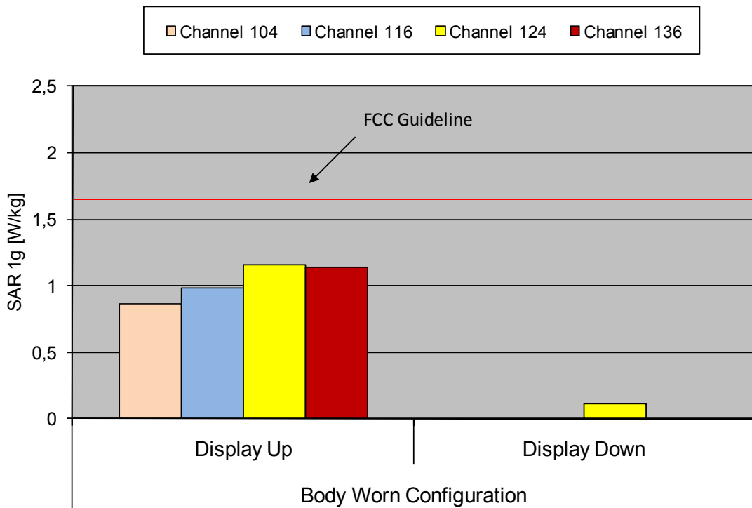
Fig. 19: The measured body SAR values for IEEE 802.11 n (5.5 GHz range) for the Ascom WH1-EACA/PF in body worn configuration, in comparison to the FCC exposure limit.
