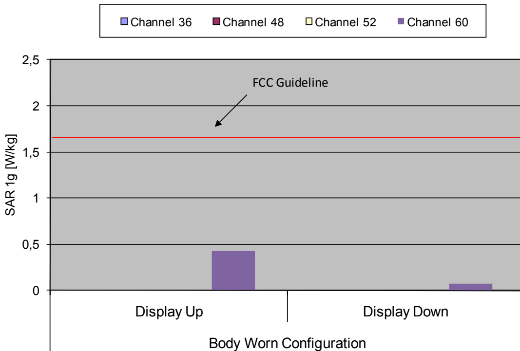
Fig. 15: The measured body SAR values for IEEE 802.11 n (5.2 GHz range) for the Ascom WH1-EACA/PF in body worn configuration, in comparison to the FCC exposure limit.
