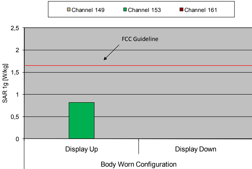
Fig. 22: The measured body SAR values for IEEE 802.11 a (5.8 GHz range) for the Ascom WH1-EACA/PF in body worn configuration, in comparison to the FCC exposure limit.
