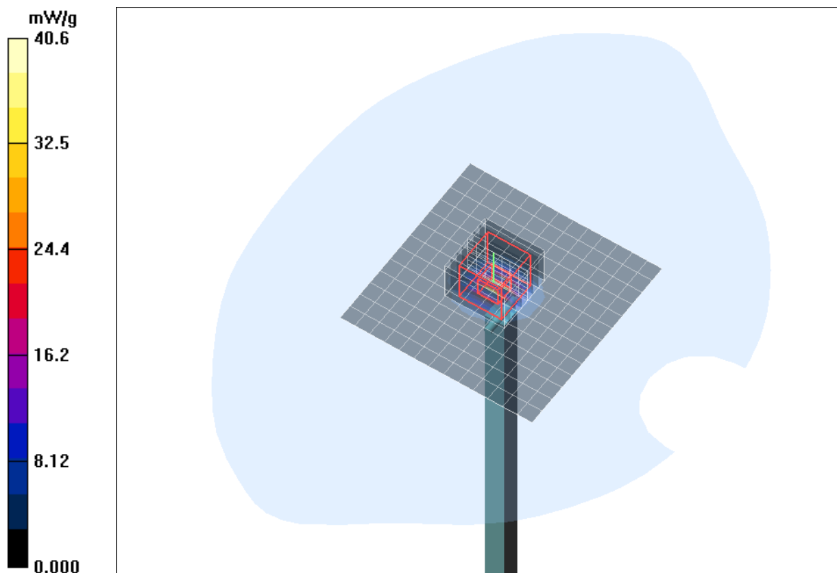
Fig. 26: Validation measurement 5200 MHz Head (August 24, 2010), coarse grid. Ambient Temperature: 22.0° C, Liquid Temperature: 21.5° C.
