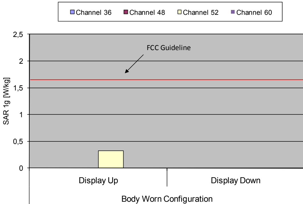
Fig. 14: The measured body SAR values for IEEE 802.11 a (5.2 GHz range) for the Ascom WH1-EACA/PF in body worn configuration, in comparison to the FCC exposure limit.
