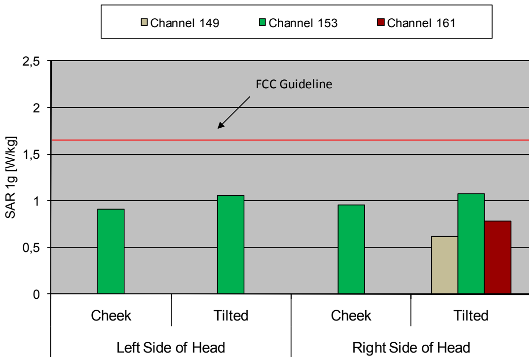
Fig. 21: The measured head SAR values for IEEE 802.11 n (5.8 GHz range) for the Ascom WH1-EACA/PF in head configuration, in comparison to the FCC exposure limit.
