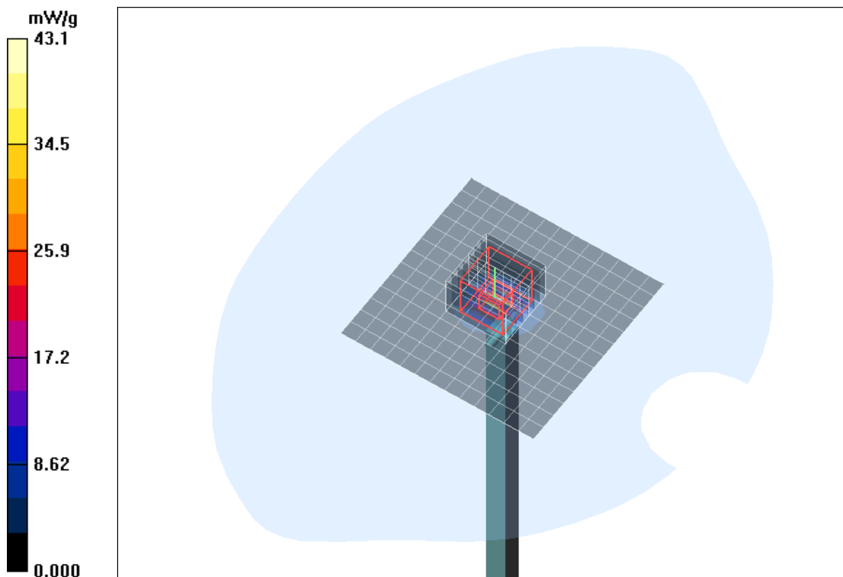
Fig. 28: Validation measurement 5500 MHz Head (August 23, 2010), coarse grid. Ambient Temperature: 22.0° C, Liquid Temperature: 21.6° C.
