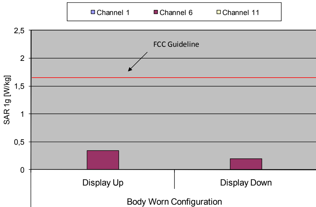
Fig. 10: The measured body SAR values for IEEE 802.11 b for the Ascom WH1-EACA/PF in body worn configuration, in comparison to the FCC exposure limit.
