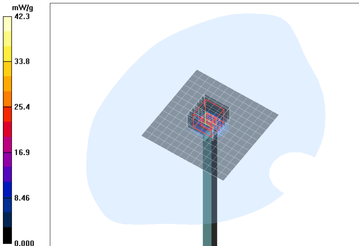
Fig. 30: Validation measurement 5800 MHz Head (August 19, 2010), coarse grid. Ambient Temperature: 22.3° C, Liquid Temperature: 21.7° C.
