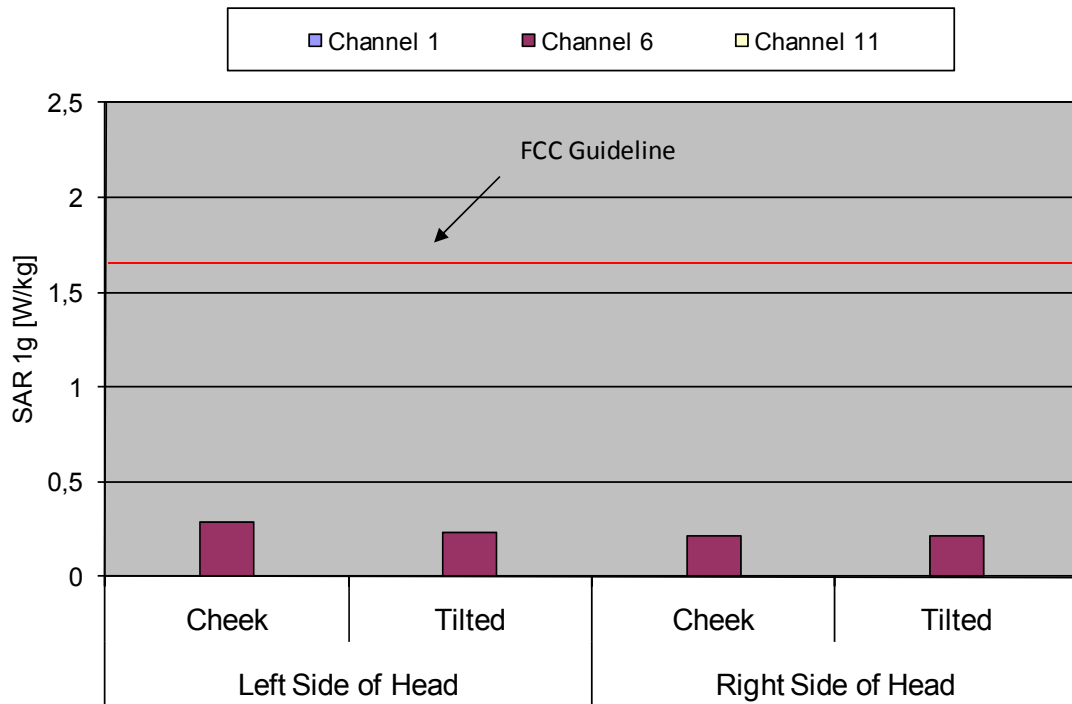
Fig. 8: The measured head SAR values for IEEE 802.11 b for the Ascom WH1-EACA/PF in head configuration, in comparison to the FCC exposure limit.
