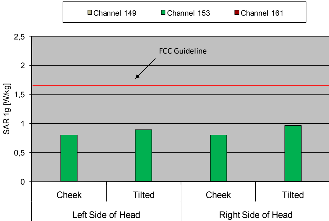
Fig. 20: The measured head SAR values for IEEE 802.11 a (5.8 GHz range) for the Ascom WH1-EACA/PF in head configuration, in comparison to the FCC exposure limit.
