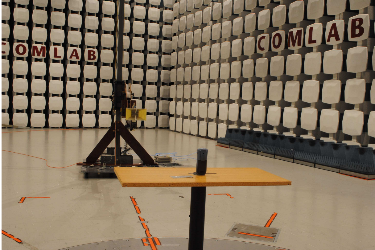
Radiated Output Power / Radiated Emissions test
