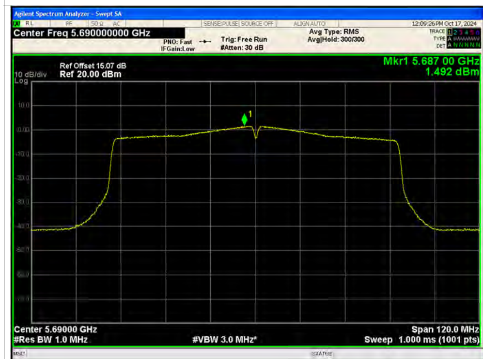
PSD NVNT ac80 5690MHz Ant2 SISO
