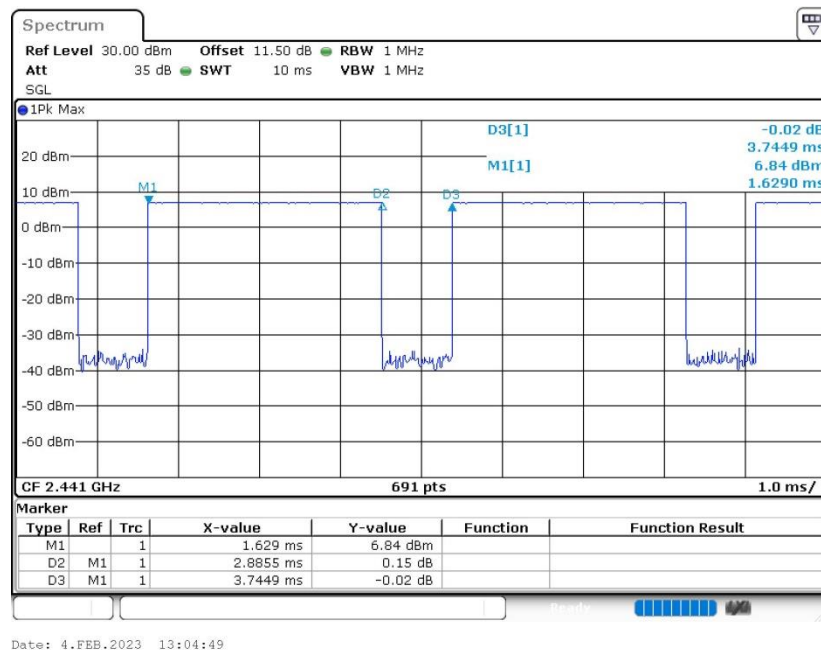
Package Transfer Time Plot-<Ant6>
