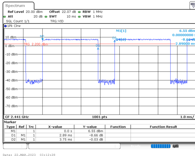
Package Transfer Time Plot-<Ant5>
