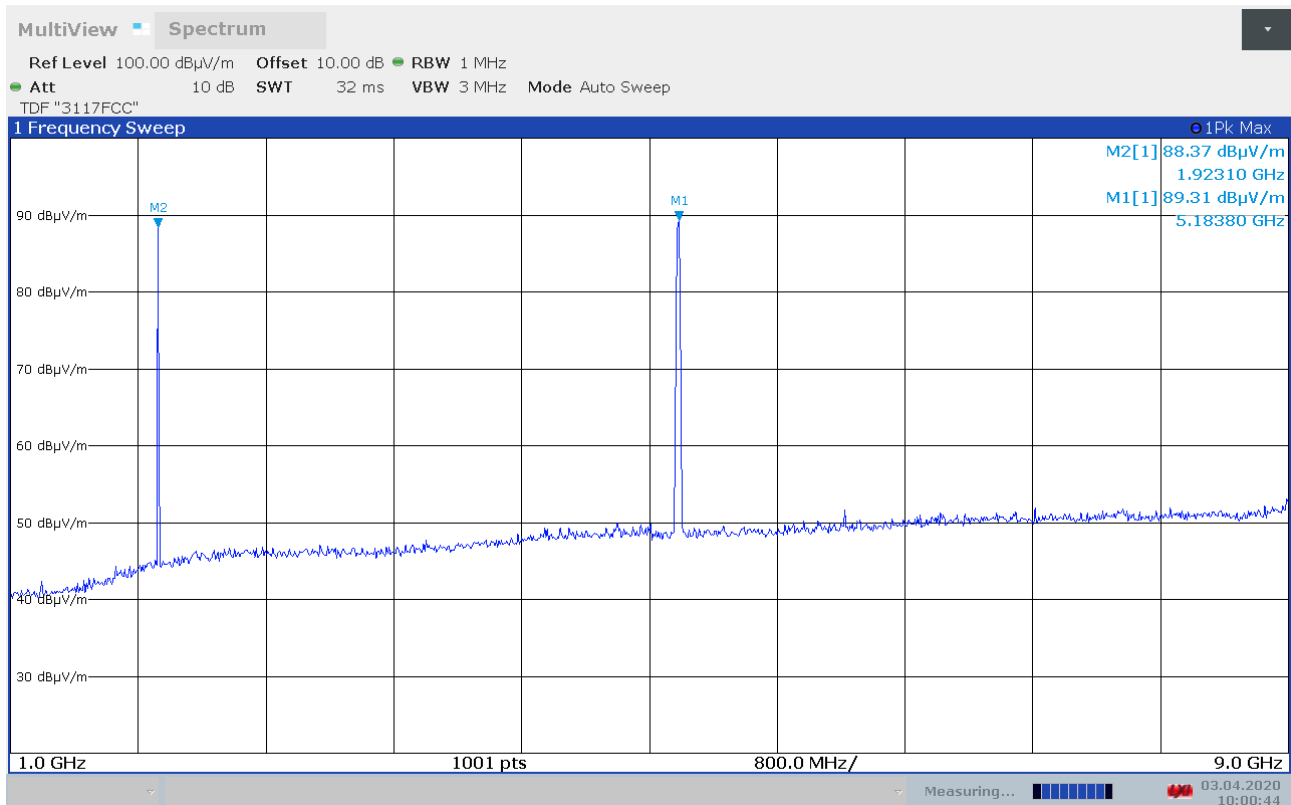
Maximum Emissions 1 – 9 GHz, DECT Ch02 + WiFi Ch36 6Mb, HP
