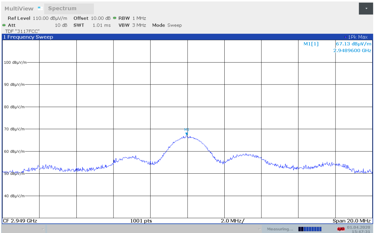
Maximum Emissions 2949 MHz, DECT Ch02 Ant 1 + WiFi Ch06 1Mb, HP
