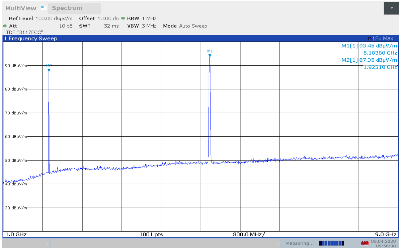
Maximum Emissions 1 – 9 GHz, DECT Ch02 + WiFi Ch36 6Mb, VP
