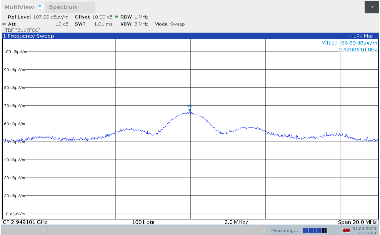
Maximum Emissions 2949 MHz, DECT Ch02 Ant 0 + WiFi Ch06 1Mb, HP
