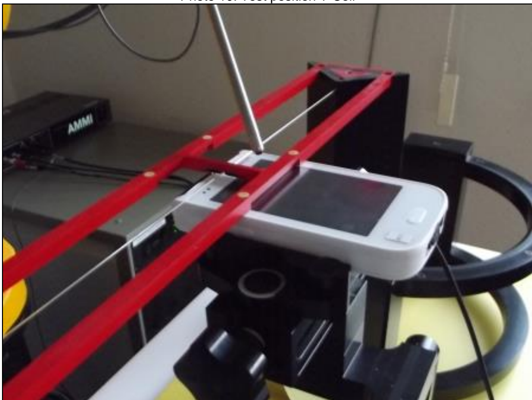
Photo 10: Test position T-Coil
