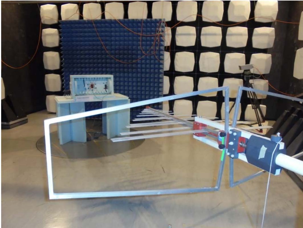
Test setup GPS mode, long shot view
