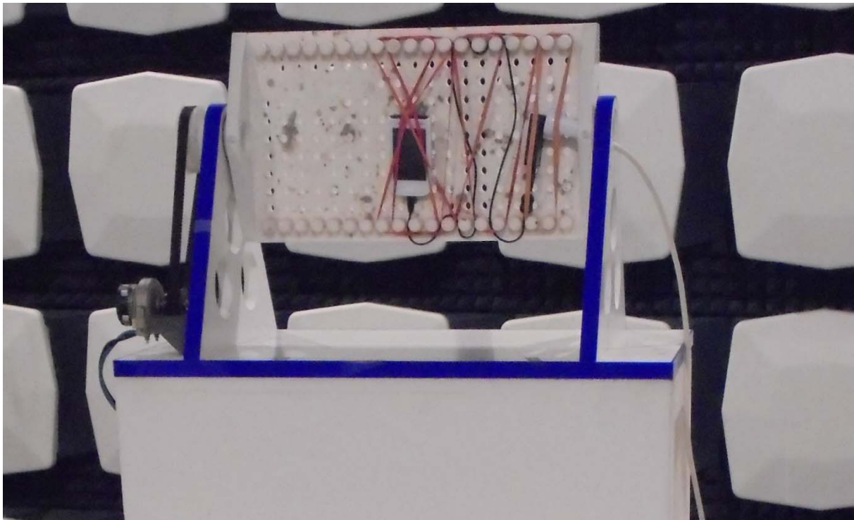
Test set-up GPS mode, close up view
