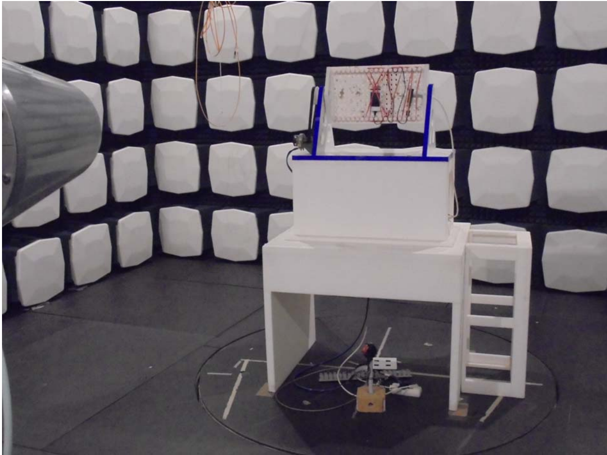
Test set-up GPS mode, long shot view
