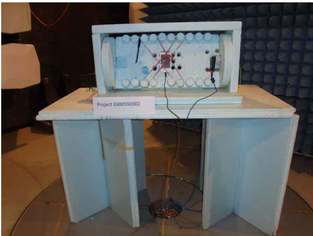
Test setup GPS mode, close-up view
