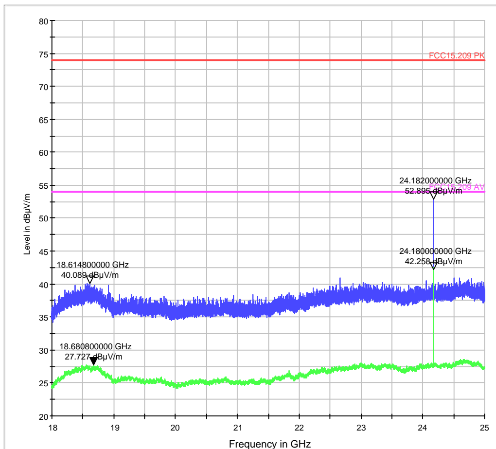
EMI Scan_18_25GHz_Pre
