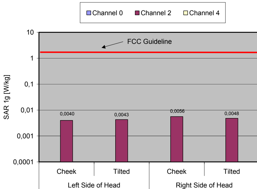
Fig. 8: The measured head phantom SAR values for the Ascom RAID2, with antenna 1 for the US DECT standard in comparison to the FCC exposure limit.
