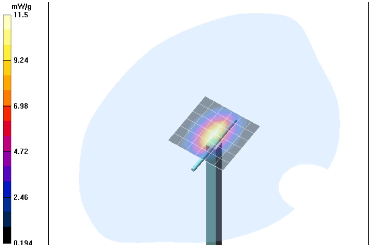
Fig. 12: Validation measurement 1900 MHz body (February 07, 2006), coarse grid. Ambient Temperature: 22.0° C, Liquid Temperature: 21.5° C.
