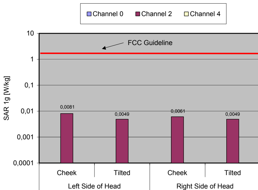
Fig. 9: The measured head phantom SAR values for the Ascom RAID2, with antenna 2 for the US DECT standard in comparison to the FCC exposure limit.
