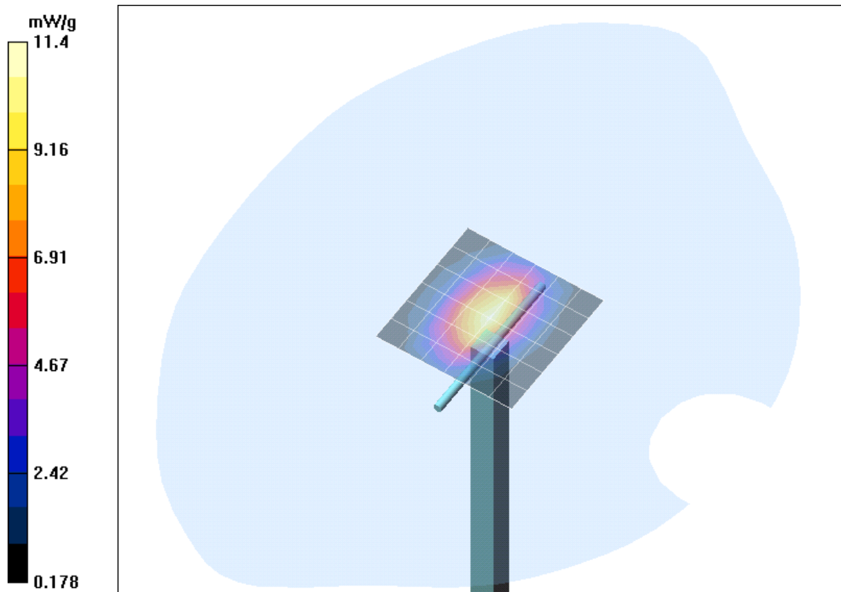
Fig. 11: Validation measurement 1900 MHz Head (February 06, 2006), coarse grid. Ambient Temperature: 22.1° C, Liquid Temperature: 21.5° C.
