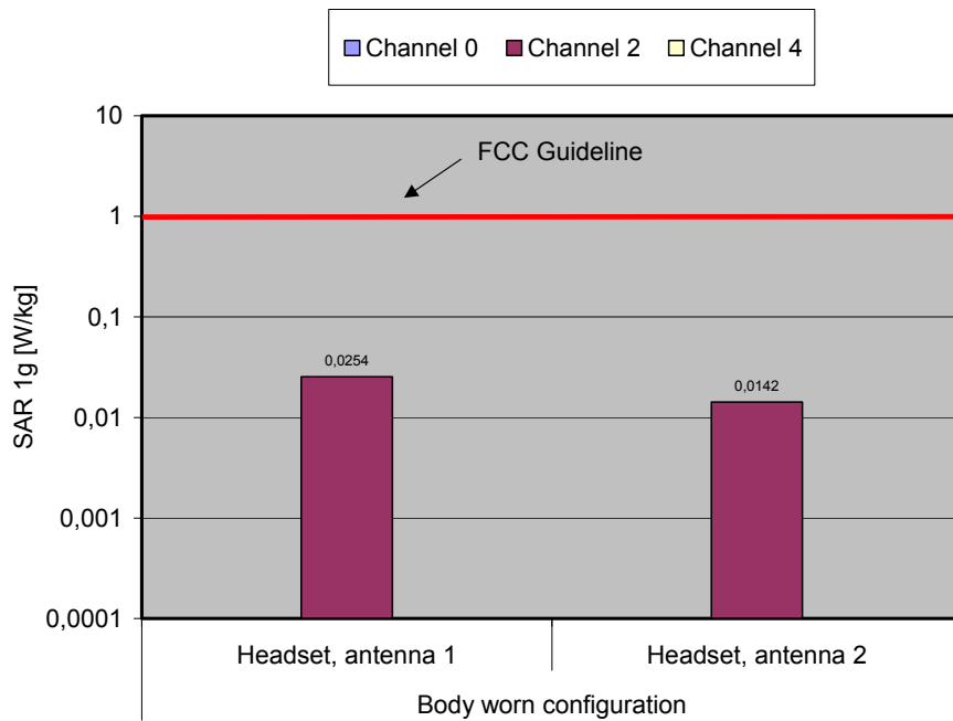
Fig. 10: The measured SAR values in body-worn configuration for the Ascom RAID2 for the US DECT standard in comparison to the FCC exposure limit.
