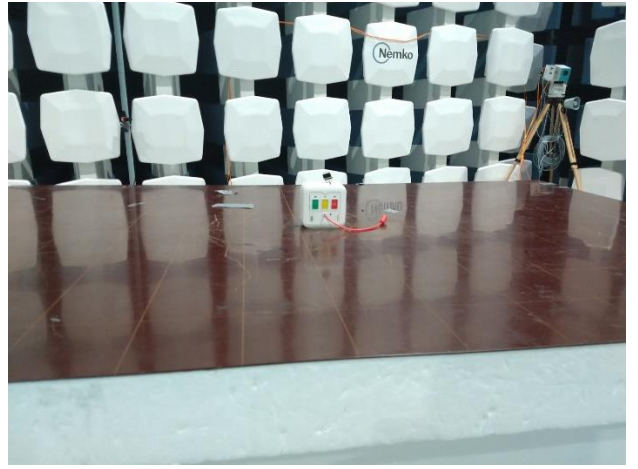
Test setup , XZ Plane
