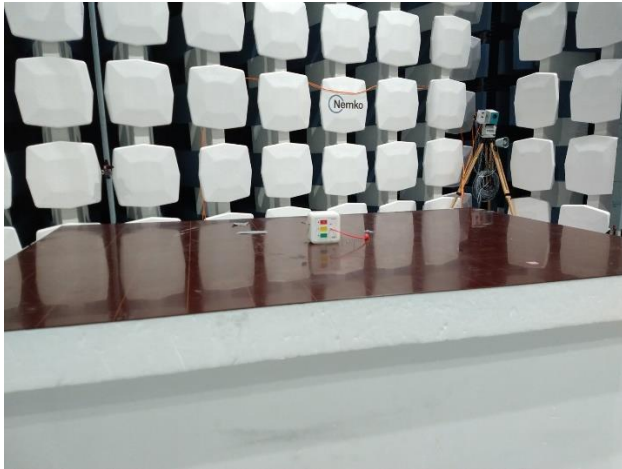
Test setup , YZ Plane
