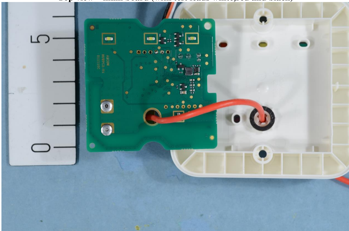
Rear view – main board (with test leads white,red and black)
