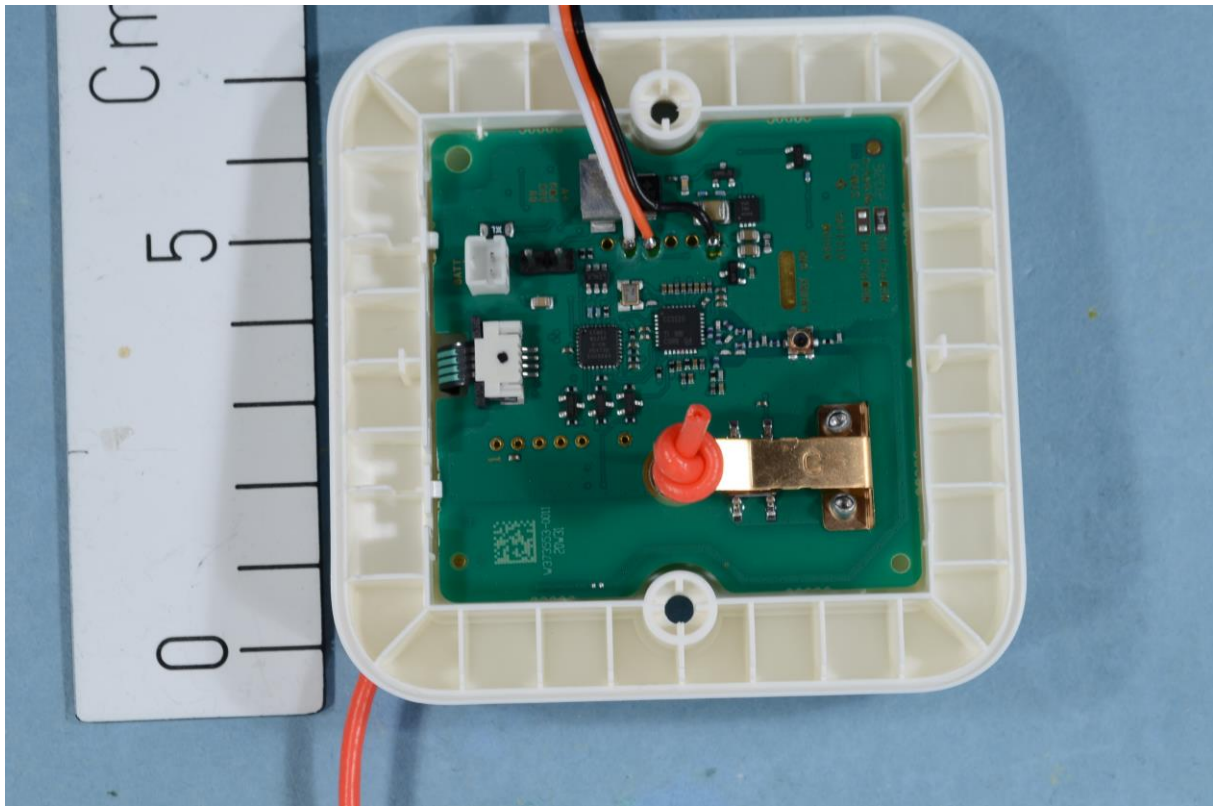
Top view – main board (with test leads white,red and black)
