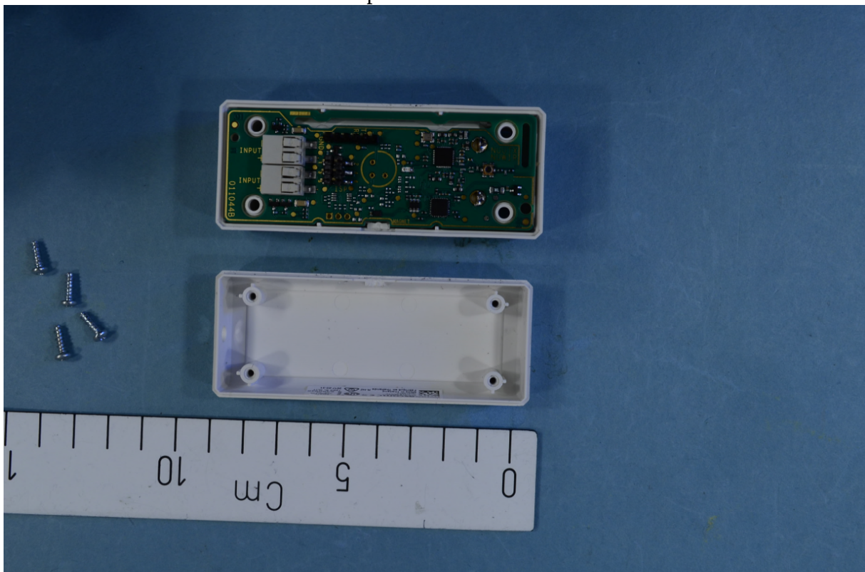
Top view – NUUTX (only difference is sensor from NUWIR)
