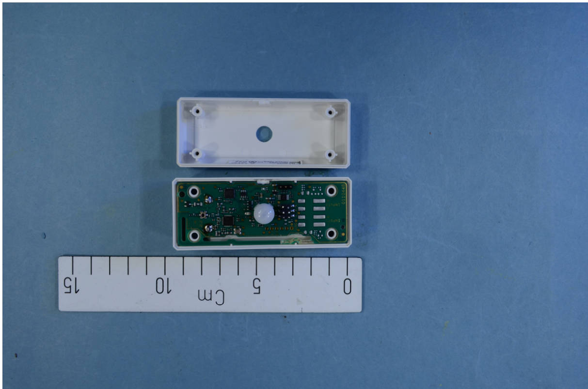
Top view – NUWIR
